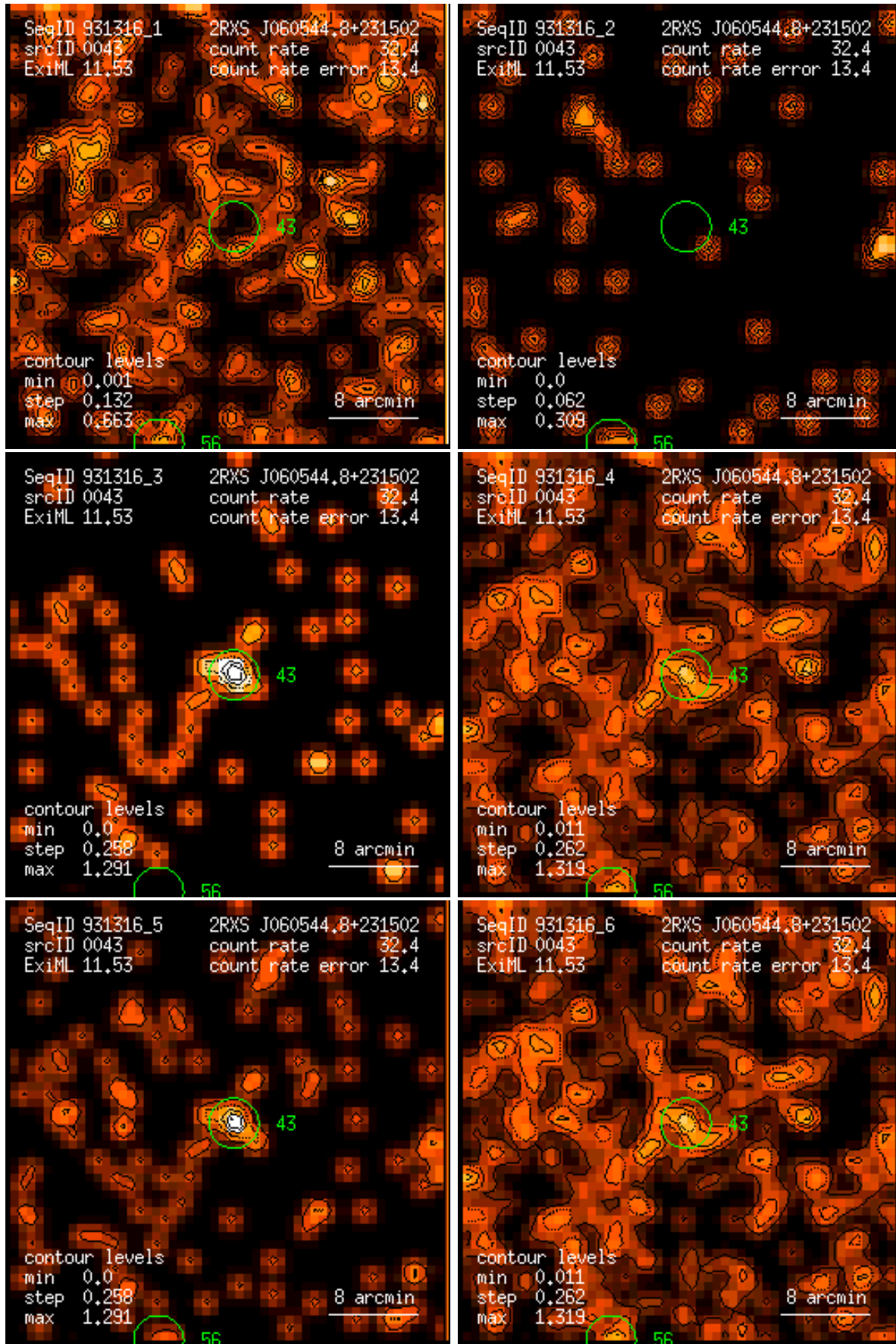
Figure 43: RASS 931316: detection 0043: band rate images, Gaussian filter: (1) PSPC channels 11 – 41, (2) 52 – 90, (3) 91 – 201, (4) 11 – 235, (5) 52 – 201, (6) 11 – 201. Broad band rates in counts/ks. Band rate contour levels in counts/ks/arcmin 2 .
