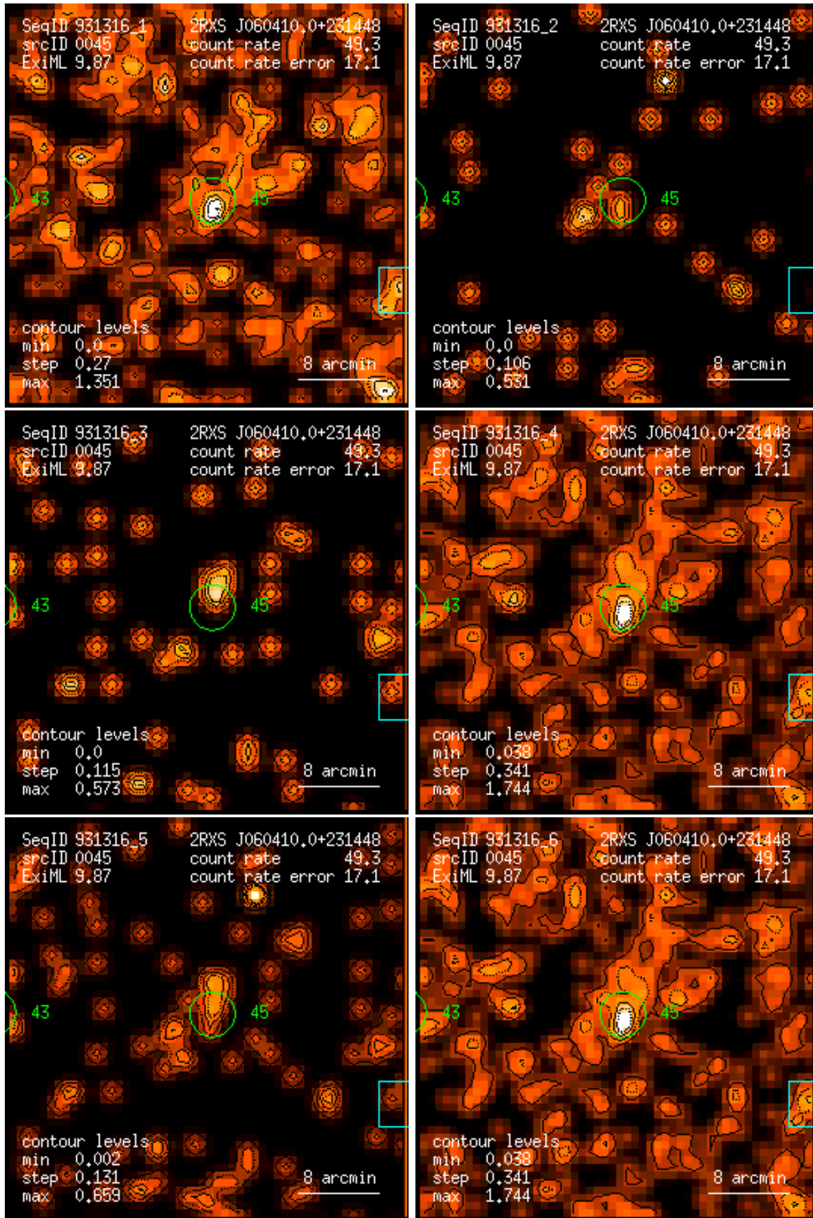
Figure 45: RASS 931316: detection 0045: band rate images, Gaussian filter: (1) PSPC channels 11 – 41, (2) 52 – 90, (3) 91 – 201, (4) 11 – 235, (5) 52 – 201, (6) 11 – 201. Broad band rates in counts/ks. Band rate contour levels in counts/ks/arcmin 2 .
