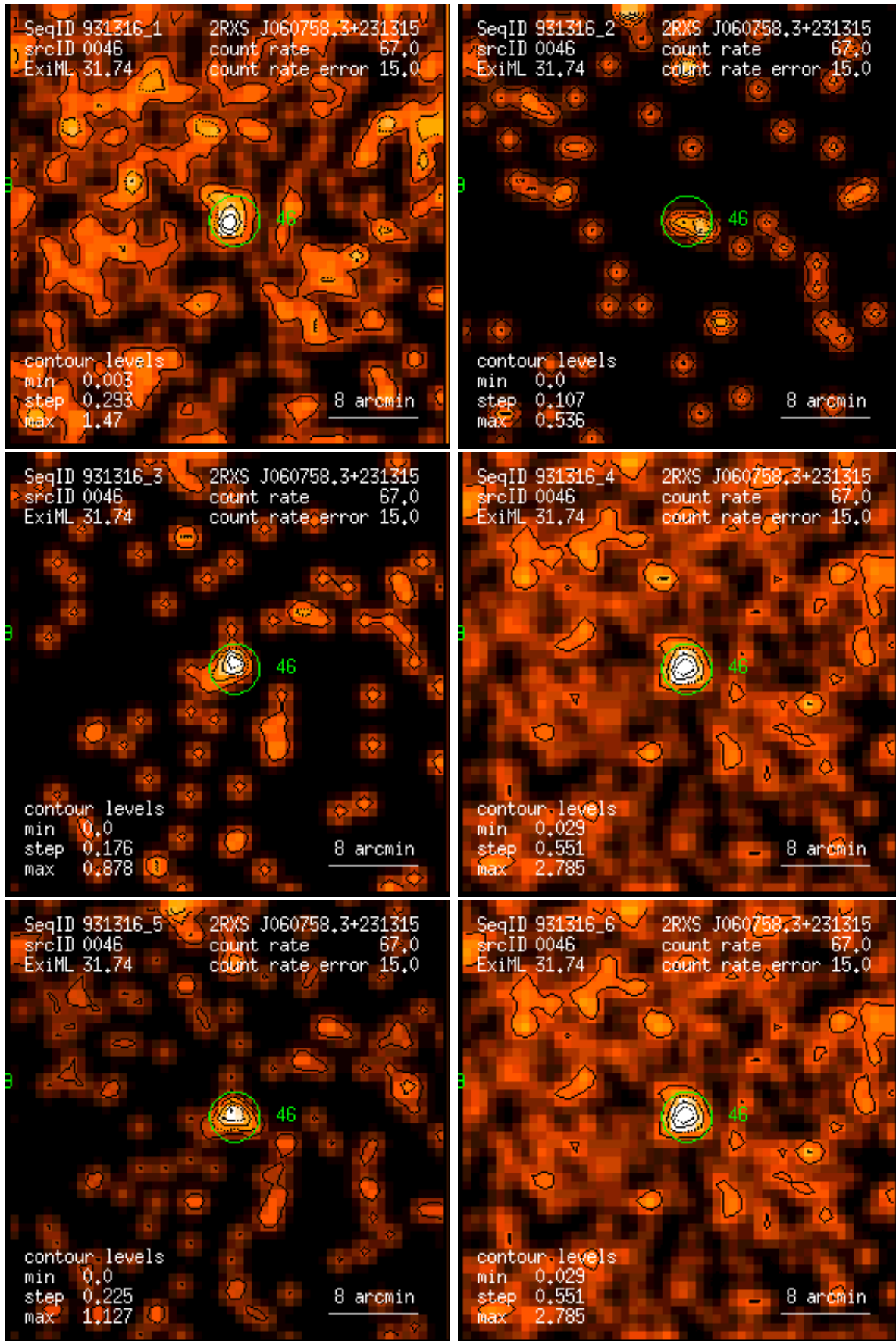
Figure 46: RASS 931316: detection 0046: band rate images, Gaussian filter: (1) PSPC channels 11 – 41, (2) 52 – 90, (3) 91 – 201, (4) 11 – 235, (5) 52 – 201, (6) 11 – 201. Broad band rates in counts/ks. Band rate contour levels in counts/ks/arcmin 2 .
