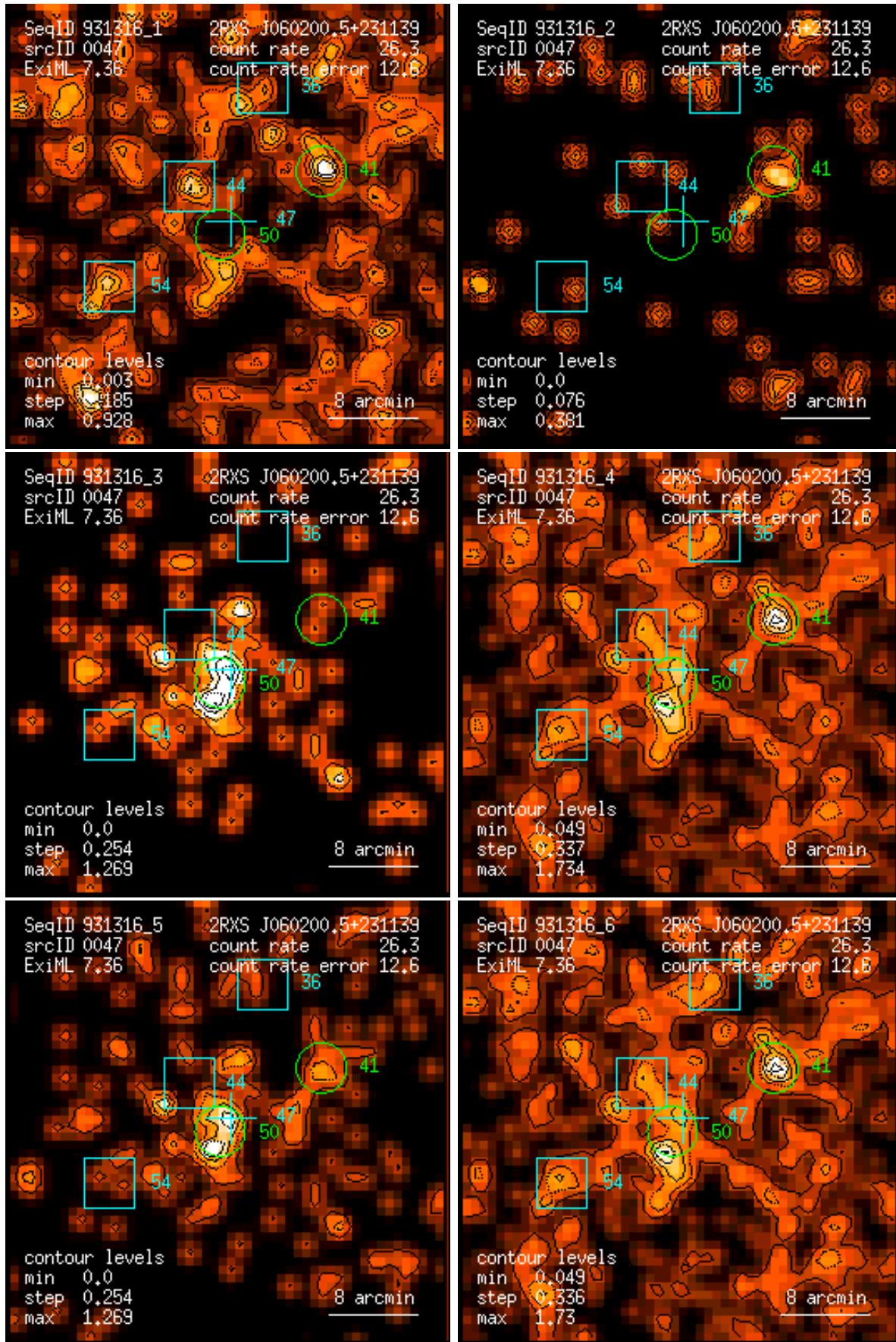
Figure 47: RASS 931316: detection 0047: band rate images, Gaussian filter: (1) PSPC channels 11 – 41, (2) 52 – 90, (3) 91 – 201, (4) 11 – 235, (5) 52 – 201, (6) 11 – 201. Broad band rates in counts/ks. Band rate contour levels in counts/ks/arcmin 2 .
