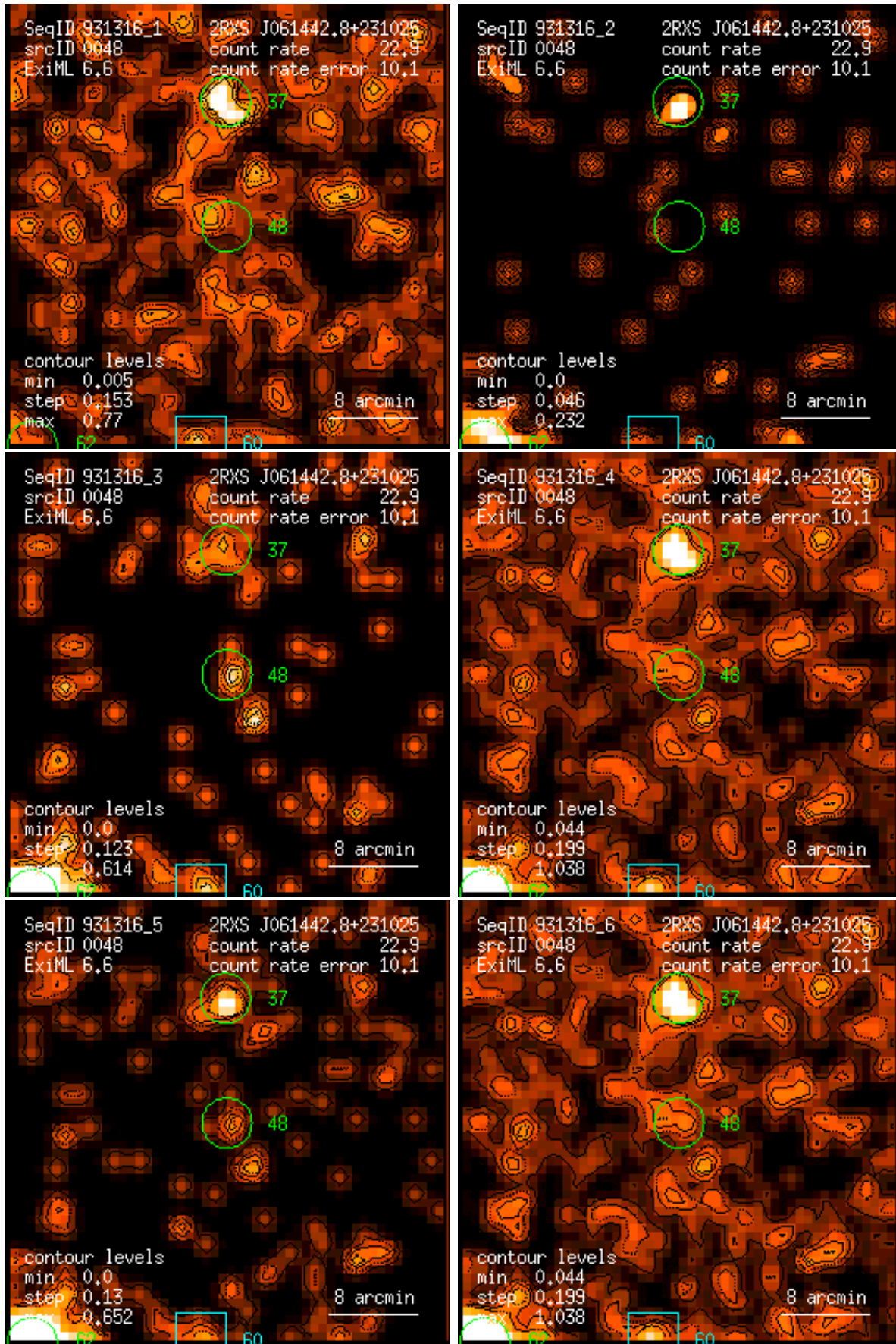
Figure 48: RASS 931316: detection 0048: band rate images, Gaussian filter: (1) PSPC channels 11 – 41, (2) 52 – 90, (3) 91 – 201, (4) 11 – 235, (5) 52 – 201, (6) 11 – 201. Broad band rates in counts/ks. Band rate contour levels in counts/ks/arcmin 2 .
