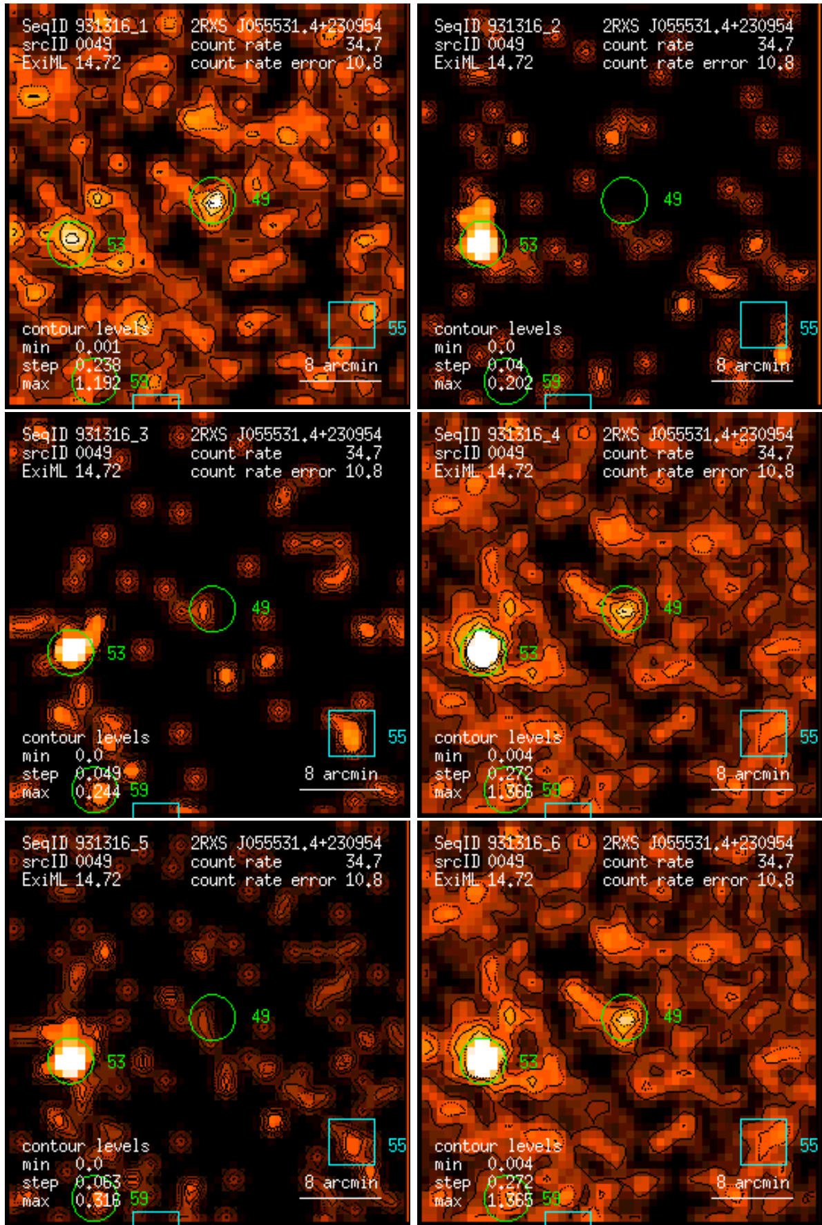
Figure 49: RASS 931316: detection 0049: band rate images, Gaussian filter: (1) PSPC channels 11 – 41, (2) 52 – 90, (3) 91 – 201, (4) 11 – 235, (5) 52 – 201, (6) 11 – 201. Broad band rates in counts/ks. Band rate contour levels in counts/ks/arcmin 2 .
