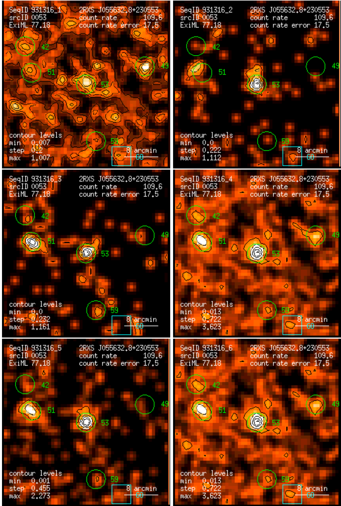
Figure 53: RASS 931316: detection 0053: band rate images, Gaussian filter: (1) PSPC channels 11 – 41, (2) 52 – 90, (3) 91 – 201, (4) 11 – 235, (5) 52 – 201, (6) 11 – 201. Broad band rates in counts/ks. Band rate contour levels in counts/ks/arcmin 2 .
