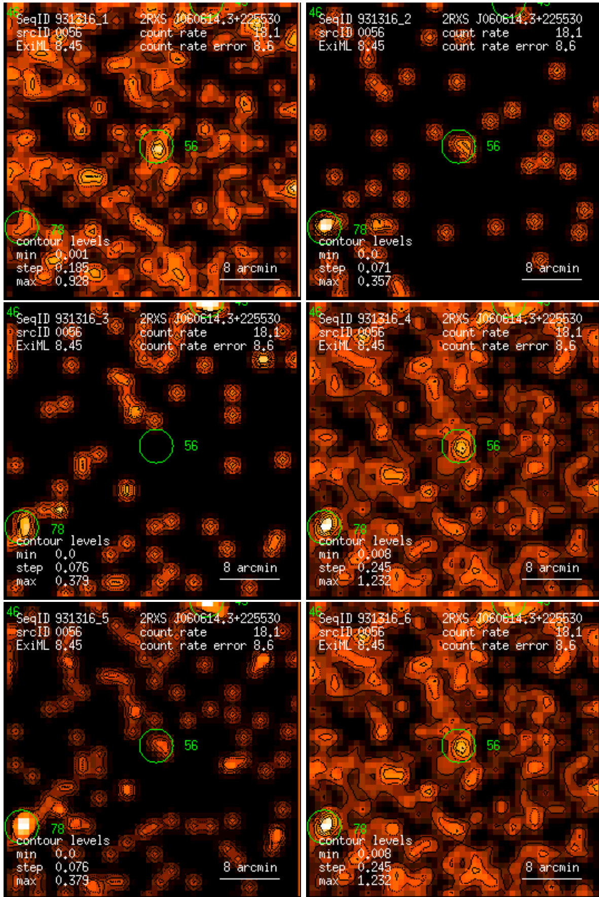
Figure 56: RASS 931316: detection 0056: band rate images, Gaussian filter: (1) PSPC channels 11 – 41, (2) 52 – 90, (3) 91 – 201, (4) 11 – 235, (5) 52 – 201, (6) 11 – 201. Broad band rates in counts/ks. Band rate contour levels in counts/ks/arcmin 2 .
