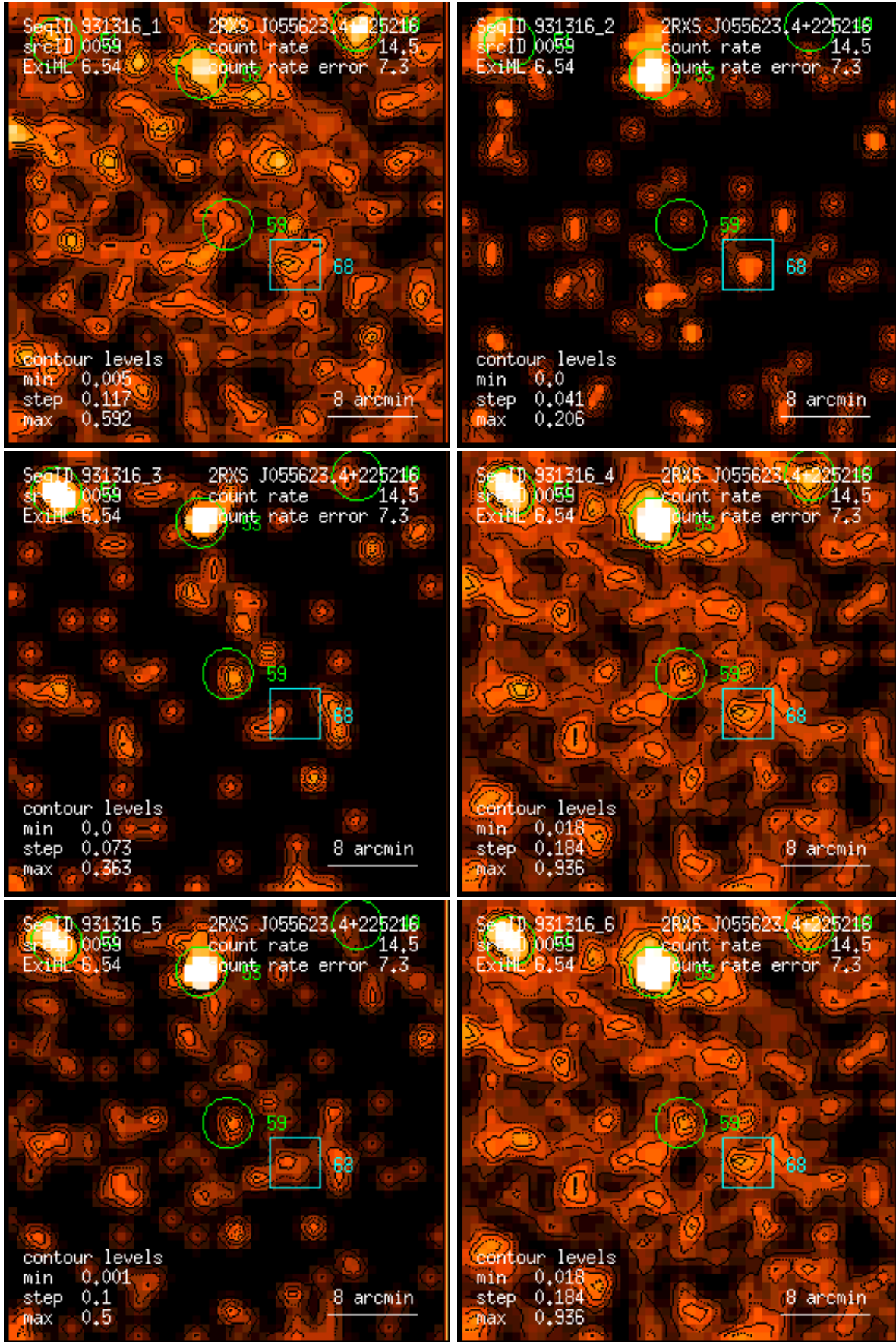
Figure 59: RASS 931316: detection 0059: band rate images, Gaussian filter: (1) PSPC channels 11 – 41, (2) 52 – 90, (3) 91 – 201, (4) 11 – 235, (5) 52 – 201, (6) 11 – 201. Broad band rates in counts/ks. Band rate contour levels in counts/ks/arcmin 2 .
