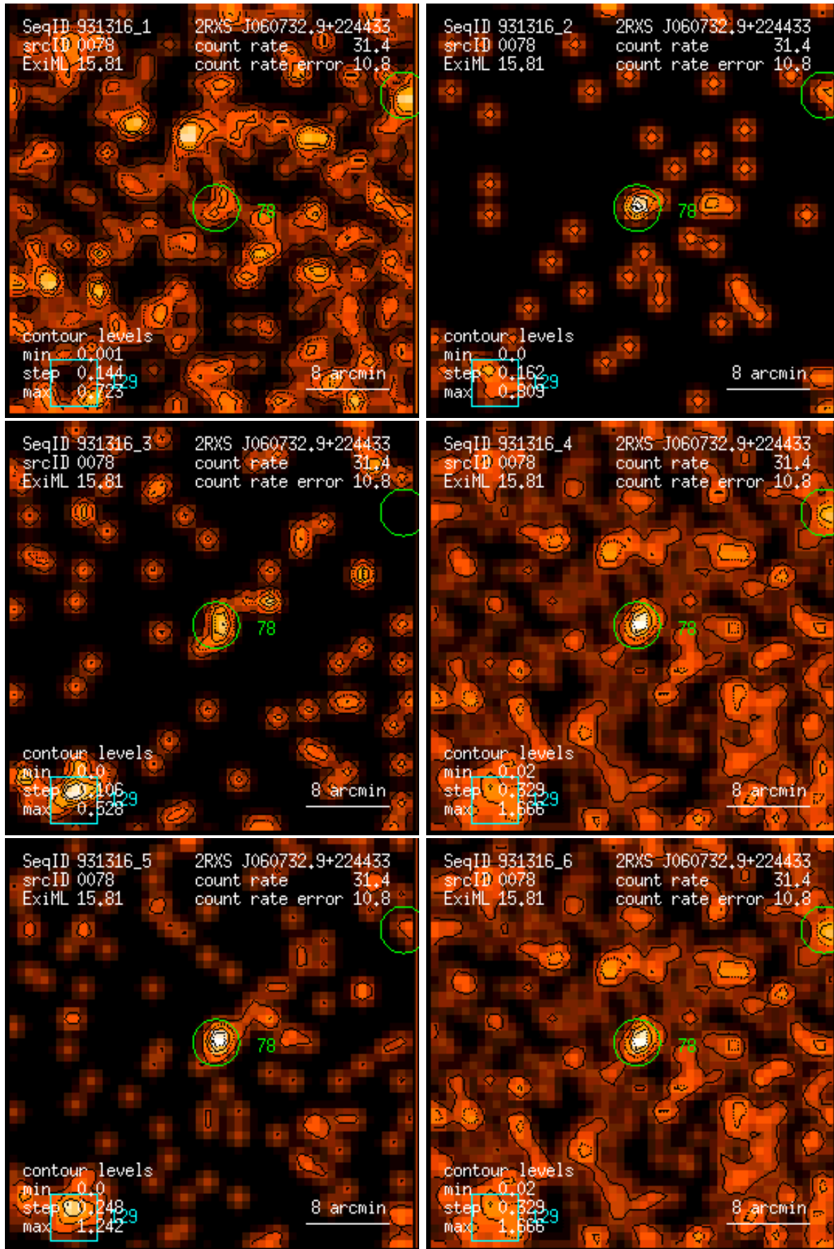
Figure 78: RASS 931316: detection 0078: band rate images, Gaussian filter: (1) PSPC channels 11 – 41, (2) 52 – 90, (3) 91 – 201, (4) 11 – 235, (5) 52 – 201, (6) 11 – 201. Broad band rates in counts/ks. Band rate contour levels in counts/ks/arcmin 2 .
