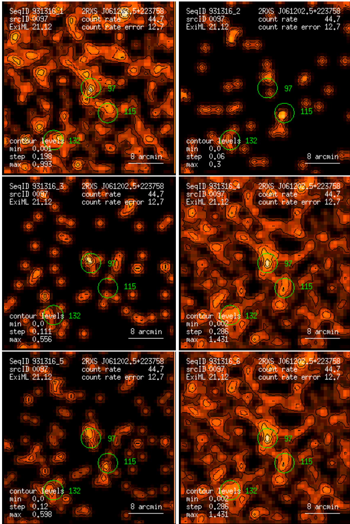
Figure 97: RASS 931316: detection 0097: band rate images, Gaussian filter: (1) PSPC channels 11 – 41, (2) 52 – 90, (3) 91 – 201, (4) 11 – 235, (5) 52 – 201, (6) 11 – 201. Broad band rates in counts/ks. Band rate contour levels in counts/ks/arcmin 2 .
