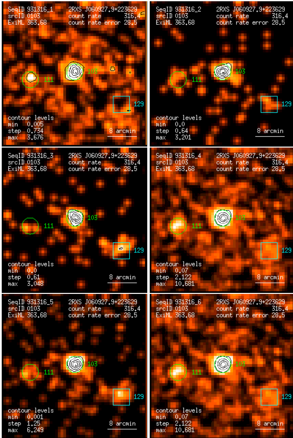
Figure 103: RASS 931316: detection 0103: band rate images, Gaussian filter: (1) PSPC channels 11 – 41, (2) 52 – 90, (3) 91 – 201, (4) 11 – 235, (5) 52 – 201, (6) 11 – 201. Broad band rates in counts/ks. Band rate contour levels in counts/ks/arcmin 2 .
