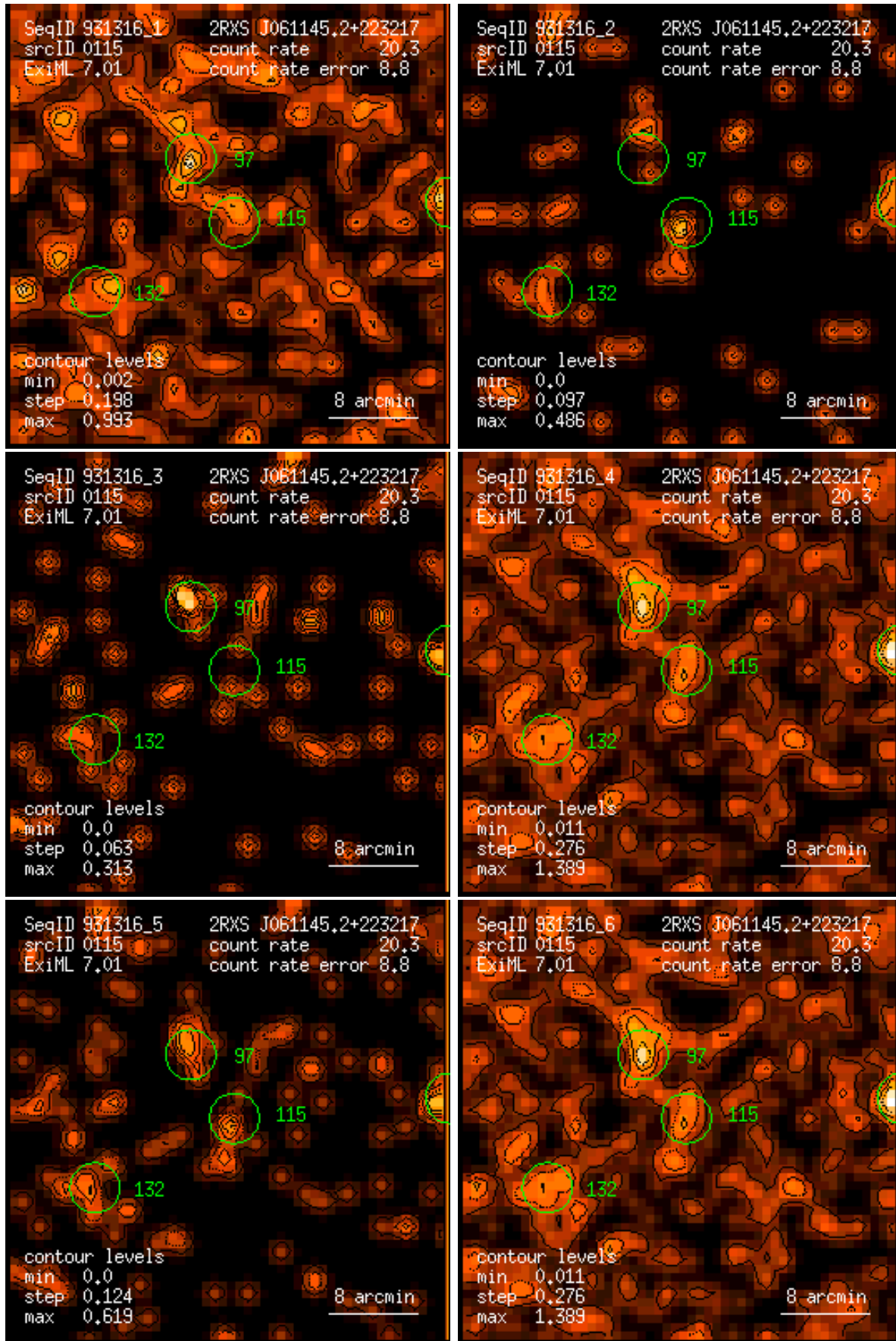
Figure 115: RASS 931316: detection 0115: band rate images, Gaussian filter: (1) PSPC channels 11 – 41, (2) 52 – 90, (3) 91 – 201, (4) 11 – 235, (5) 52 – 201, (6) 11 – 201. Broad band rates in counts/ks. Band rate contour levels in counts/ks/arcmin 2 .
