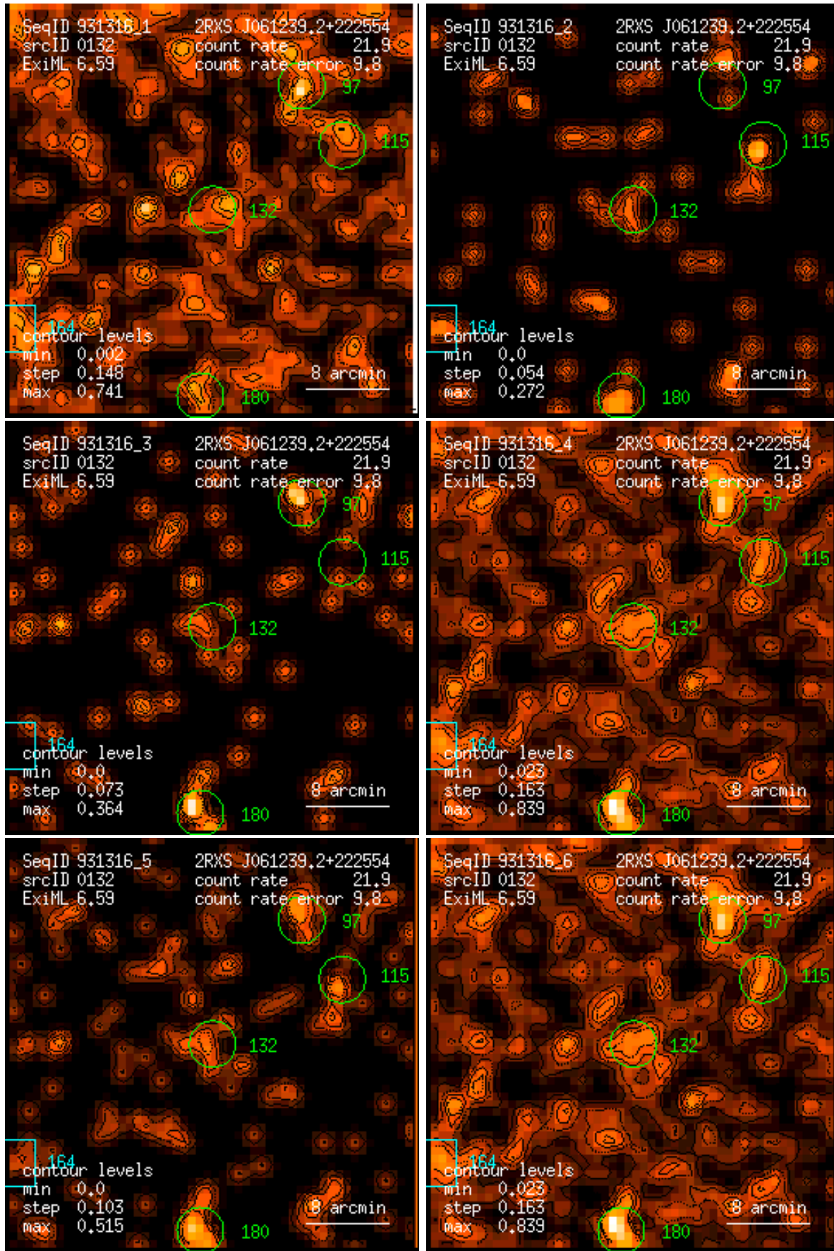
Figure 132: RASS 931316: detection 0132: band rate images, Gaussian filter: (1) PSPC channels 11 – 41, (2) 52 – 90, (3) 91 – 201, (4) 11 – 235, (5) 52 – 201, (6) 11 – 201. Broad band rates in counts/ks. Band rate contour levels in counts/ks/arcmin 2 .
