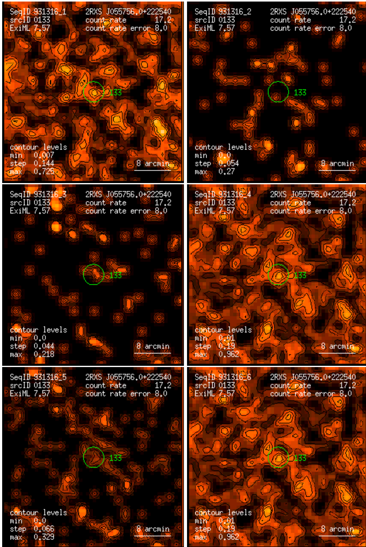
Figure 133: RASS 931316: detection 0133: band rate images, Gaussian filter: (1) PSPC channels 11 – 41, (2) 52 – 90, (3) 91 – 201, (4) 11 – 235, (5) 52 – 201, (6) 11 – 201. Broad band rates in counts/ks. Band rate contour levels in counts/ks/arcmin 2 .
