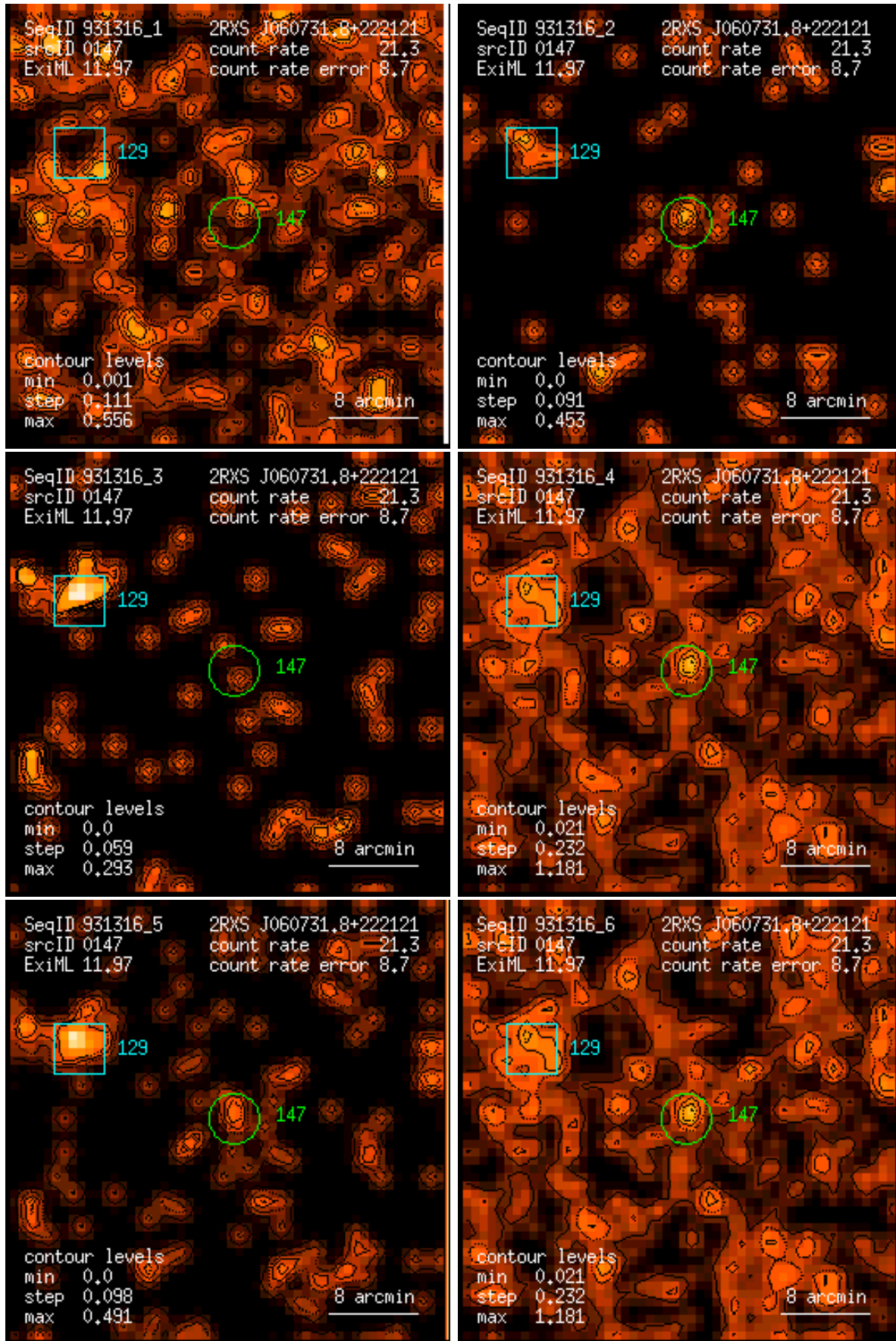
Figure 147: RASS 931316: detection 0147: band rate images, Gaussian filter: (1) PSPC channels 11 – 41, (2) 52 – 90, (3) 91 – 201, (4) 11 – 235, (5) 52 – 201, (6) 11 – 201. Broad band rates in counts/ks. Band rate contour levels in counts/ks/arcmin 2 .
