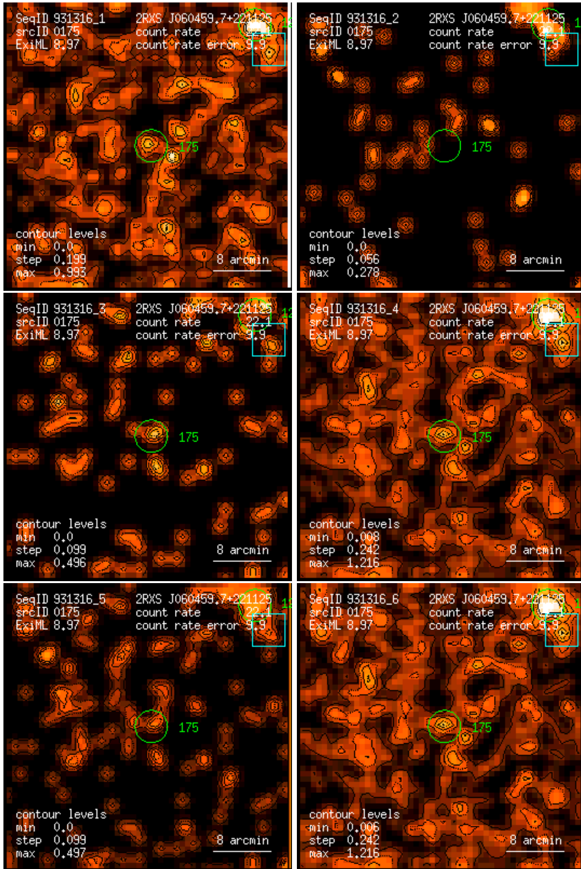
Figure 175: RASS 931316: detection 0175: band rate images, Gaussian filter: (1) PSPC channels 11 – 41, (2) 52 – 90, (3) 91 – 201, (4) 11 – 235, (5) 52 – 201, (6) 11 – 201. Broad band rates in counts/ks. Band rate contour levels in counts/ks/arcmin 2 .
