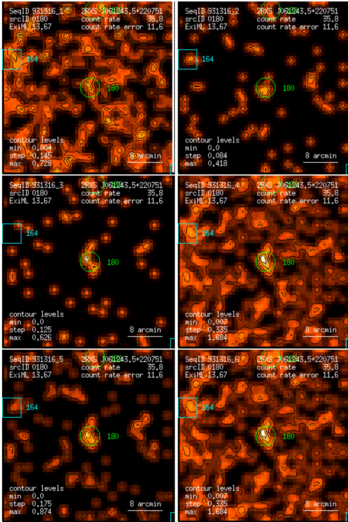
Figure 180: RASS 931316: detection 0180: band rate images, Gaussian filter: (1) PSPC channels 11 – 41, (2) 52 – 90, (3) 91 – 201, (4) 11 – 235, (5) 52 – 201, (6) 11 – 201. Broad band rates in counts/ks. Band rate contour levels in counts/ks/arcmin 2 .
