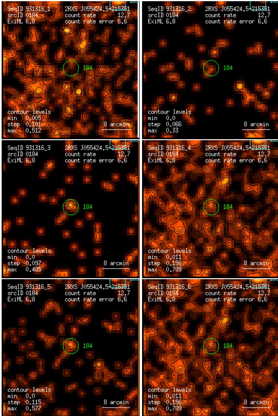
Figure 184: RASS 931316: detection 0184: band rate images, Gaussian filter: (1) PSPC channels 11 – 41, (2) 52 – 90, (3) 91 – 201, (4) 11 – 235, (5) 52 – 201, (6) 11 – 201. Broad band rates in counts/ks. Band rate contour levels in counts/ks/arcmin 2 .
