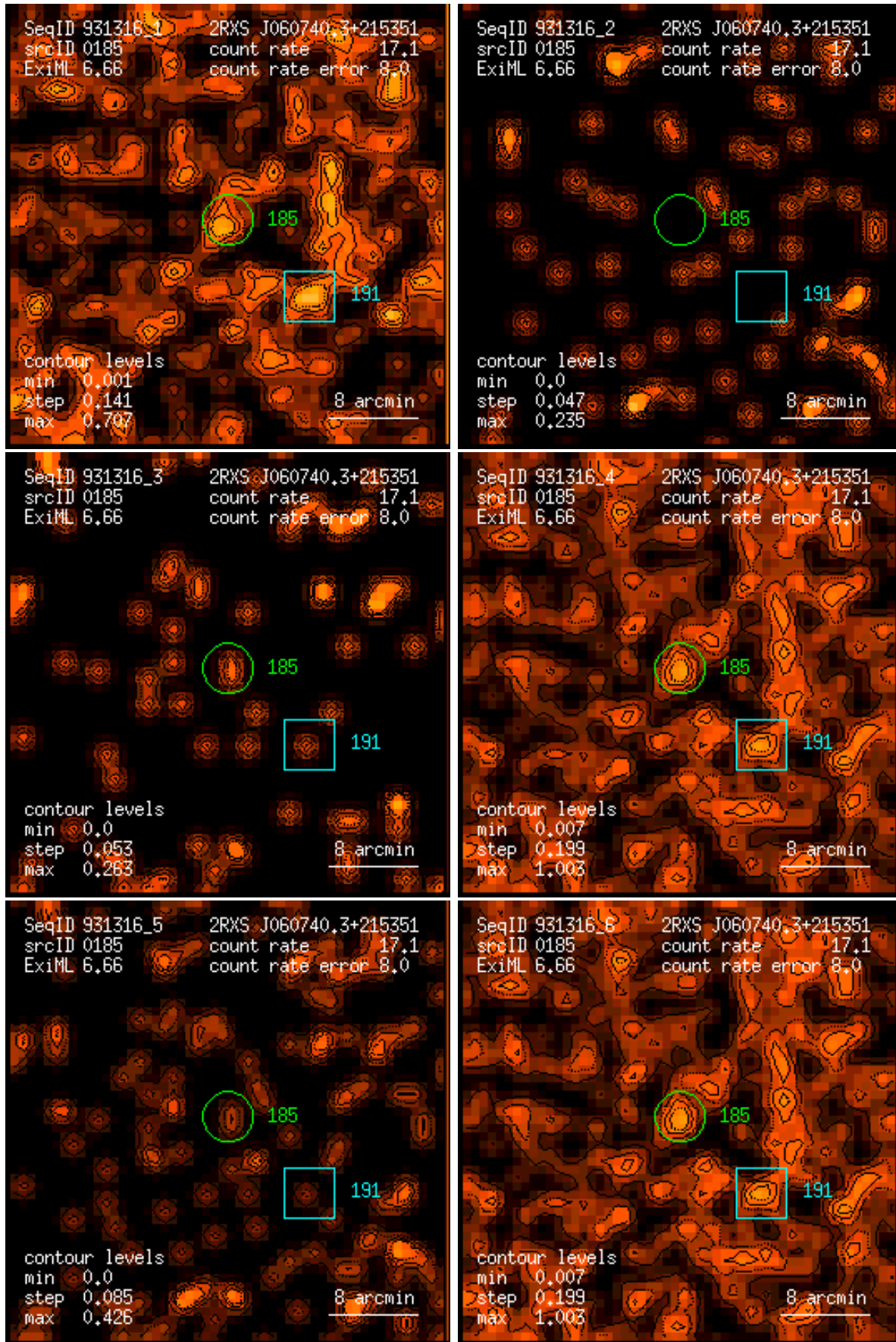
Figure 185: RASS 931316: detection 0185: band rate images, Gaussian filter: (1) PSPC channels 11 – 41, (2) 52 – 90, (3) 91 – 201, (4) 11 – 235, (5) 52 – 201, (6) 11 – 201. Broad band rates in counts/ks. Band rate contour levels in counts/ks/arcmin 2 .
