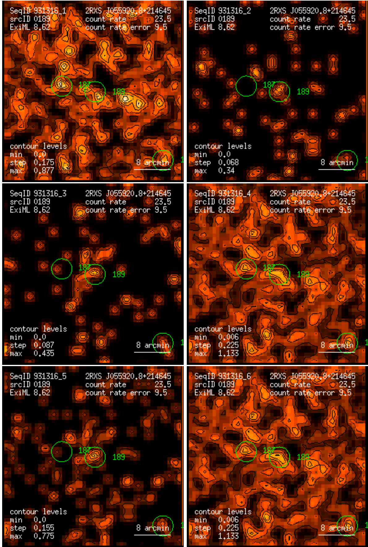
Figure 189: RASS 931316: detection 0189: band rate images, Gaussian filter: (1) PSPC channels 11 – 41, (2) 52 – 90, (3) 91 – 201, (4) 11 – 235, (5) 52 – 201, (6) 11 – 201. Broad band rates in counts/ks. Band rate contour levels in counts/ks/arcmin 2 .
