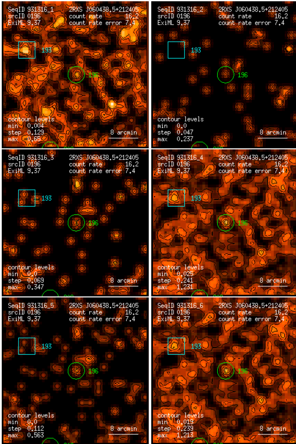
Figure 196: RASS 931316: detection 0196: band rate images, Gaussian filter: (1) PSPC channels 11 – 41, (2) 52 – 90, (3) 91 – 201, (4) 11 – 235, (5) 52 – 201, (6) 11 – 201. Broad band rates in counts/ks. Band rate contour levels in counts/ks/arcmin 2 .
