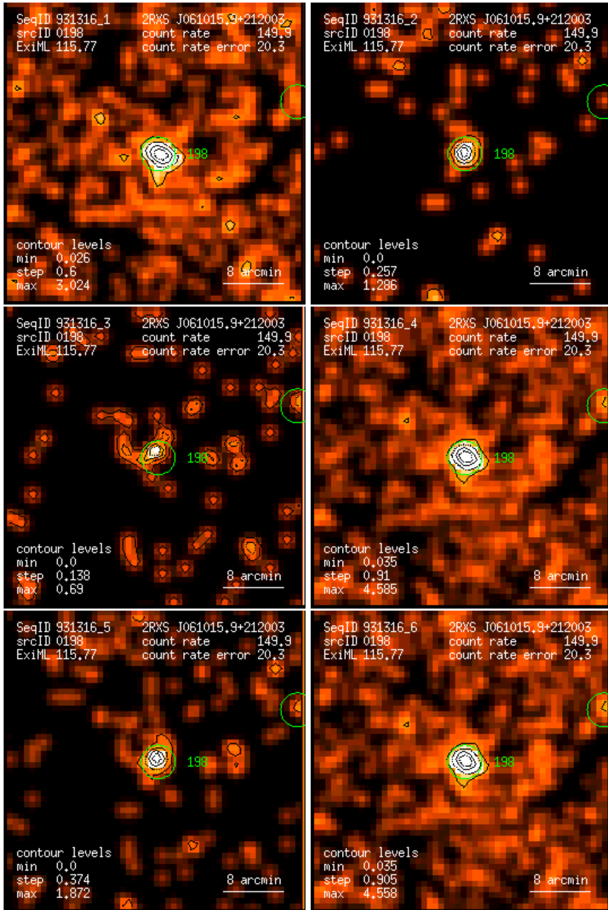
Figure 198: RASS 931316: detection 0198: band rate images, Gaussian filter: (1) PSPC channels 11 – 41, (2) 52 – 90, (3) 91 – 201, (4) 11 – 235, (5) 52 – 201, (6) 11 – 201. Broad band rates in counts/ks. Band rate contour levels in counts/ks/arcmin 2 .
