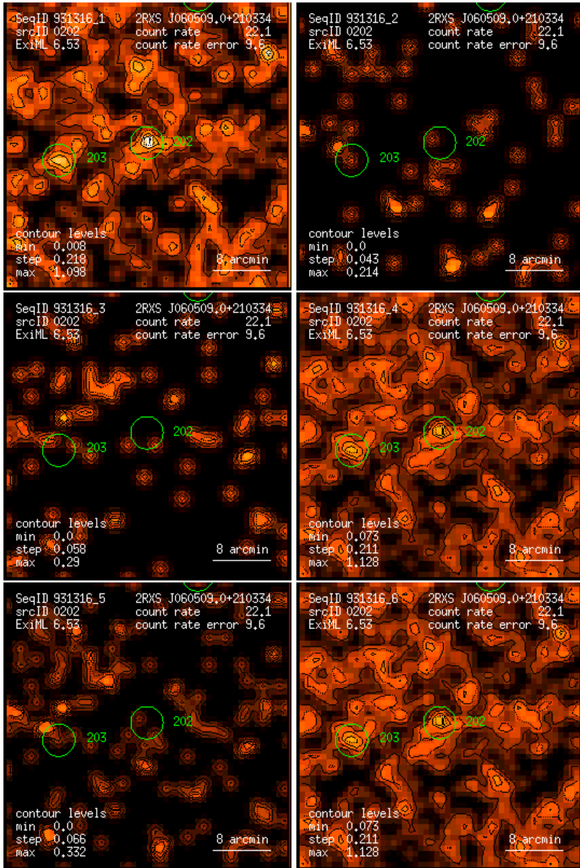
Figure 202: RASS 931316: detection 0202: band rate images, Gaussian filter: (1) PSPC channels 11 – 41, (2) 52 – 90, (3) 91 – 201, (4) 11 – 235, (5) 52 – 201, (6) 11 – 201. Broad band rates in counts/ks. Band rate contour levels in counts/ks/arcmin 2 .
