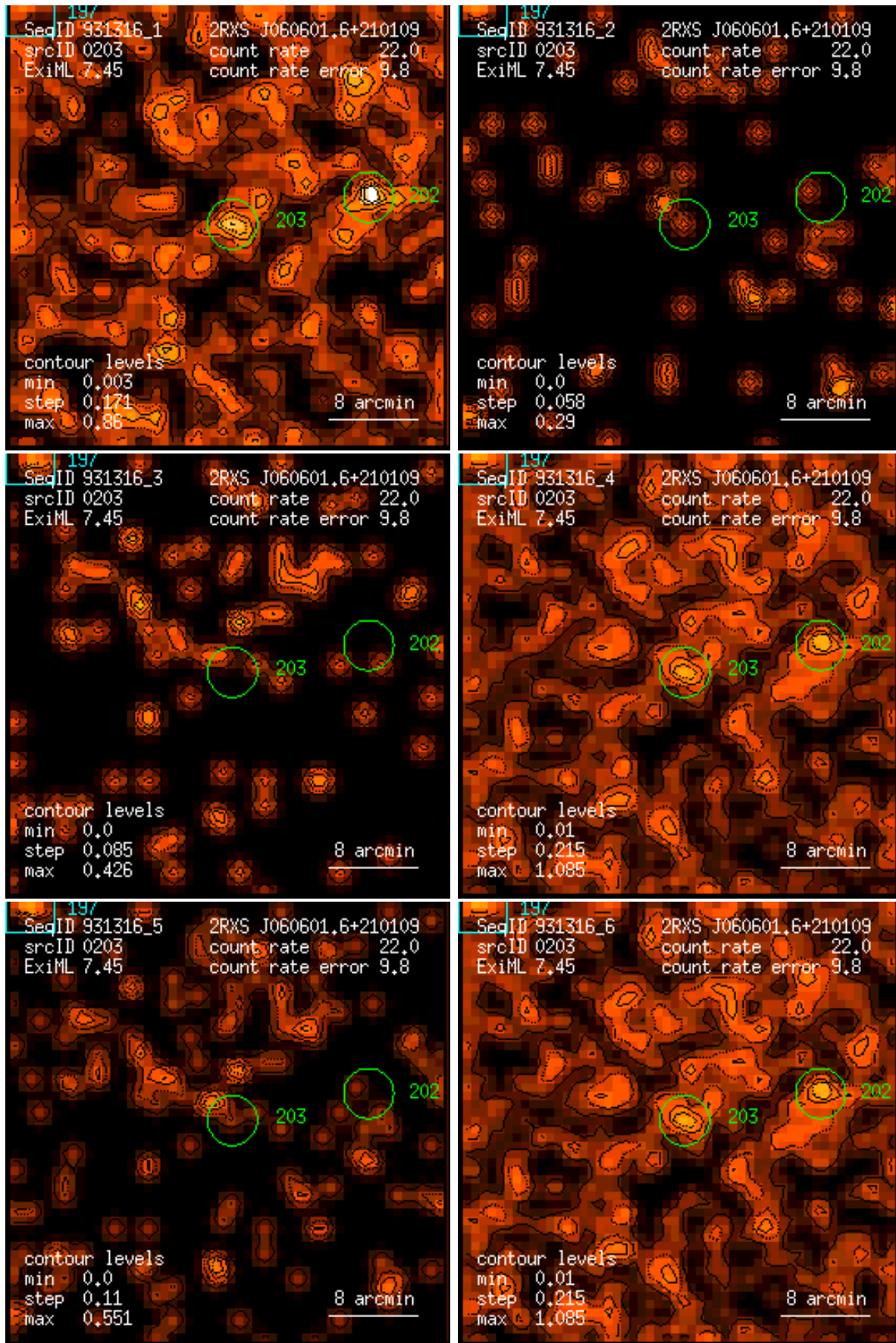
Figure 203: RASS 931316: detection 0203: band rate images, Gaussian filter: (1) PSPC channels 11 – 41, (2) 52 – 90, (3) 91 – 201, (4) 11 – 235, (5) 52 – 201, (6) 11 – 201. Broad band rates in counts/ks. Band rate contour levels in counts/ks/arcmin 2 .
