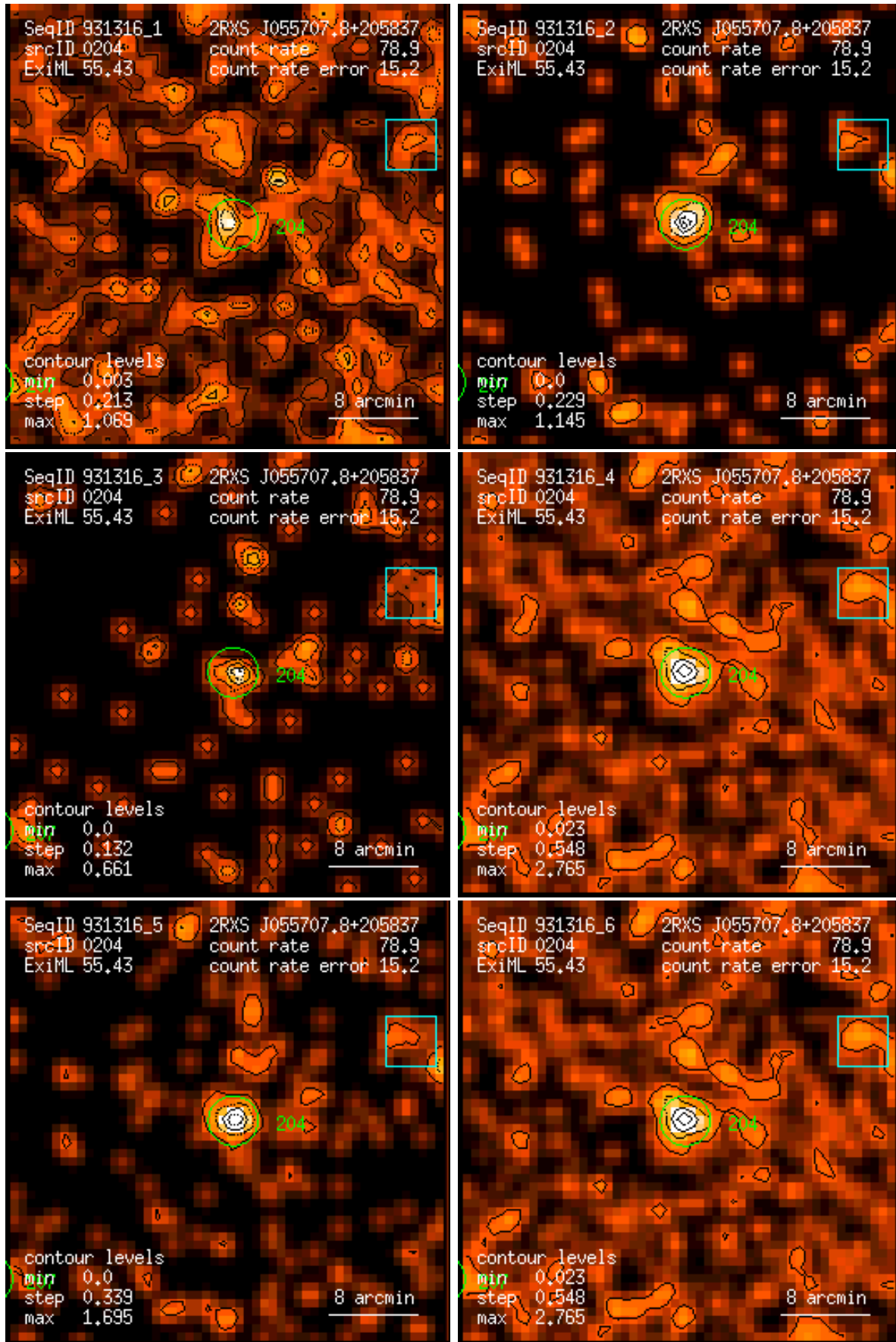
Figure 204: RASS 931316: detection 0204: band rate images, Gaussian filter: (1) PSPC channels 11 – 41, (2) 52 – 90, (3) 91 – 201, (4) 11 – 235, (5) 52 – 201, (6) 11 – 201. Broad band rates in counts/ks. Band rate contour levels in counts/ks/arcmin 2 .
