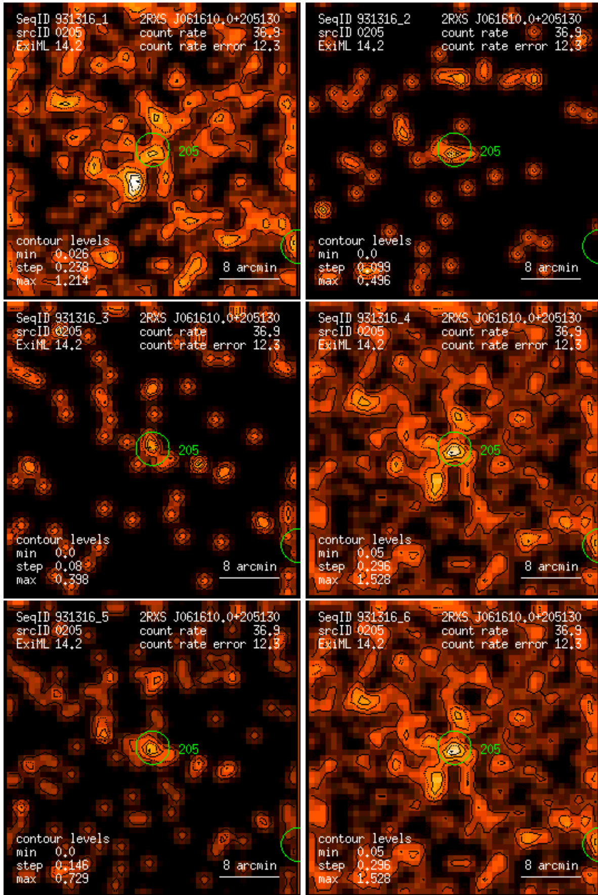
Figure 205: RASS 931316: detection 0205: band rate images, Gaussian filter: (1) PSPC channels 11 – 41, (2) 52 – 90, (3) 91 – 201, (4) 11 – 235, (5) 52 – 201, (6) 11 – 201. Broad band rates in counts/ks. Band rate contour levels in counts/ks/arcmin 2 .
