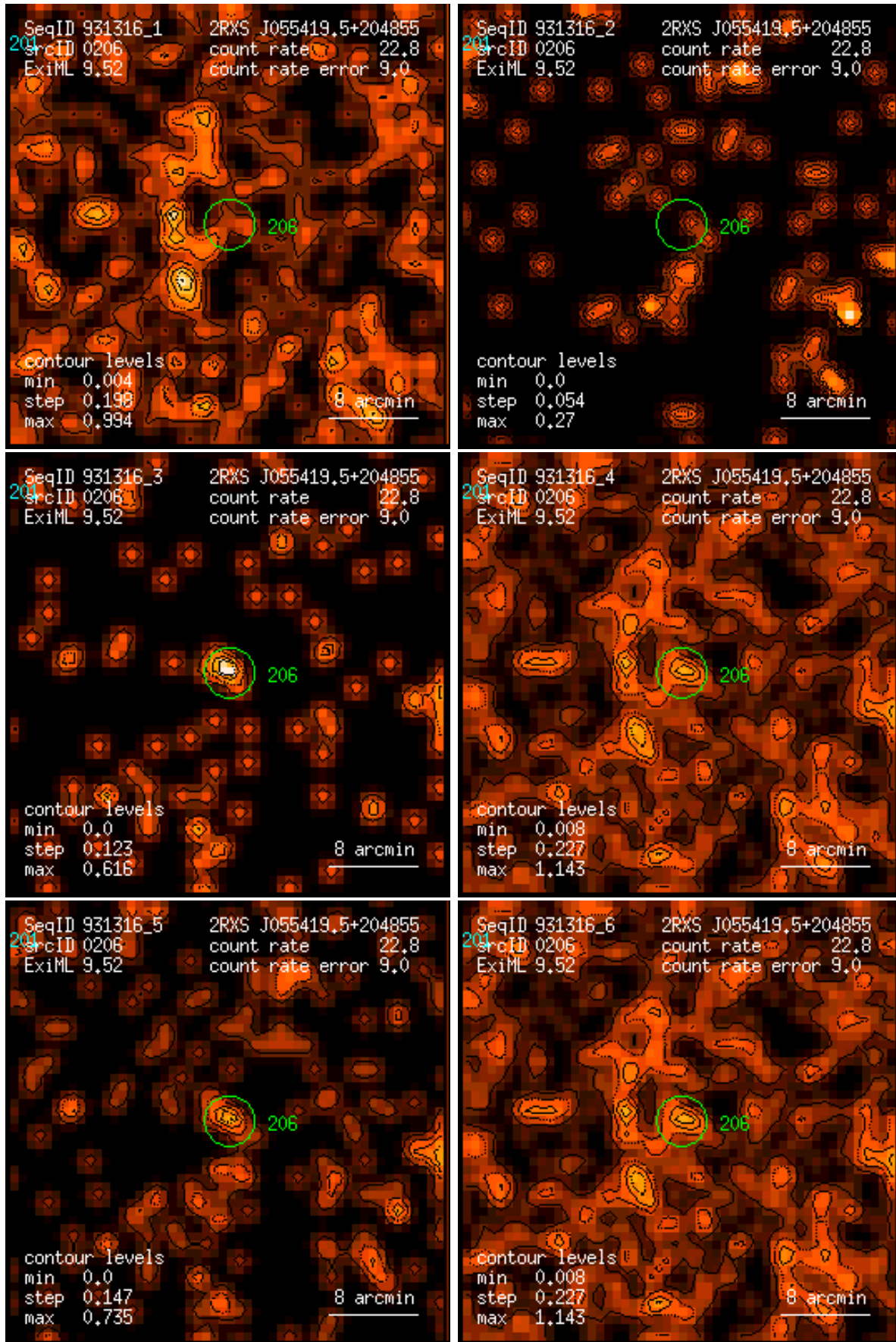
Figure 206: RASS 931316: detection 0206: band rate images, Gaussian filter: (1) PSPC channels 11 – 41, (2) 52 – 90, (3) 91 – 201, (4) 11 – 235, (5) 52 – 201, (6) 11 – 201. Broad band rates in counts/ks. Band rate contour levels in counts/ks/arcmin 2 .
