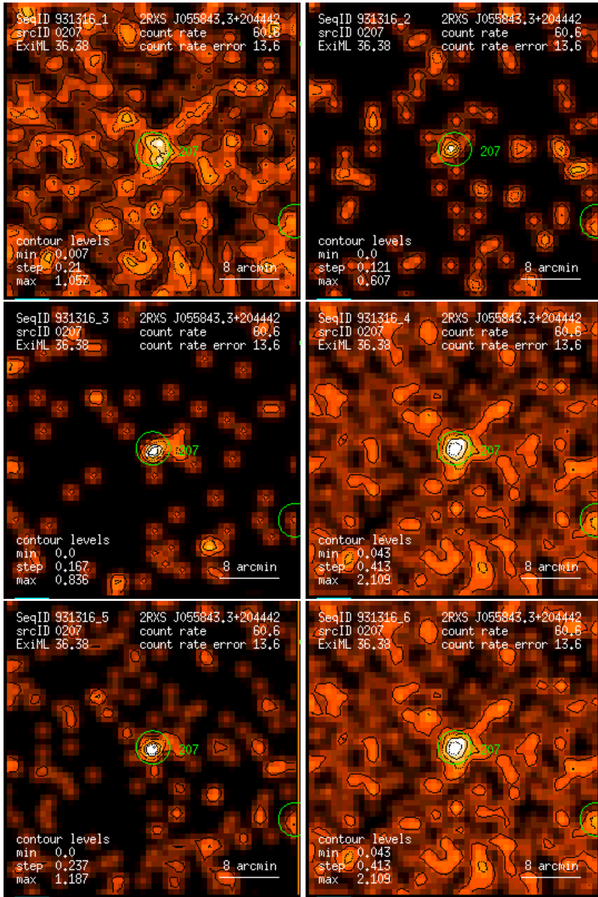
Figure 207: RASS 931316: detection 0207: band rate images, Gaussian filter: (1) PSPC channels 11 – 41, (2) 52 – 90, (3) 91 – 201, (4) 11 – 235, (5) 52 – 201, (6) 11 – 201. Broad band rates in counts/ks. Band rate contour levels in counts/ks/arcmin 2 .
