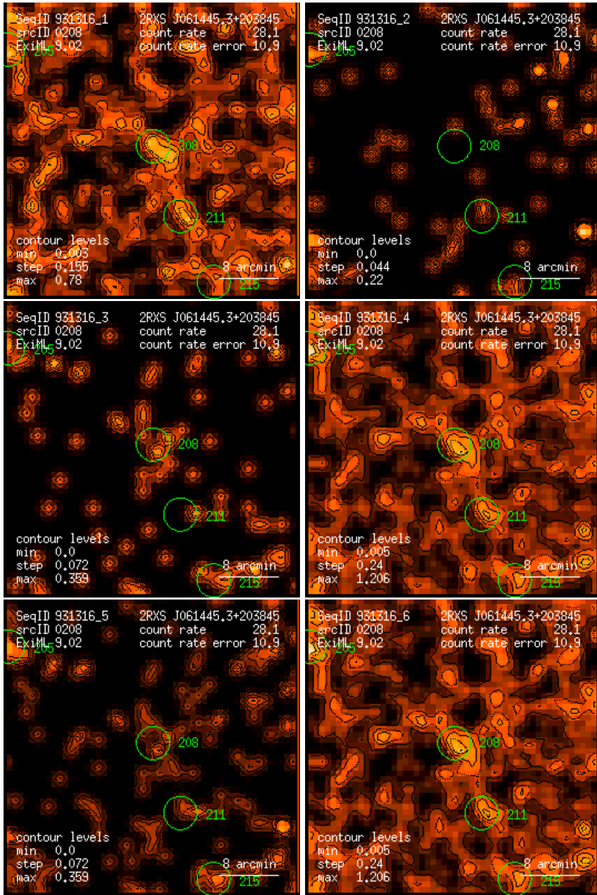
Figure 208: RASS 931316: detection 0208: band rate images, Gaussian filter: (1) PSPC channels 11 – 41, (2) 52 – 90, (3) 91 – 201, (4) 11 – 235, (5) 52 – 201, (6) 11 – 201. Broad band rates in counts/ks. Band rate contour levels in counts/ks/arcmin 2 .
