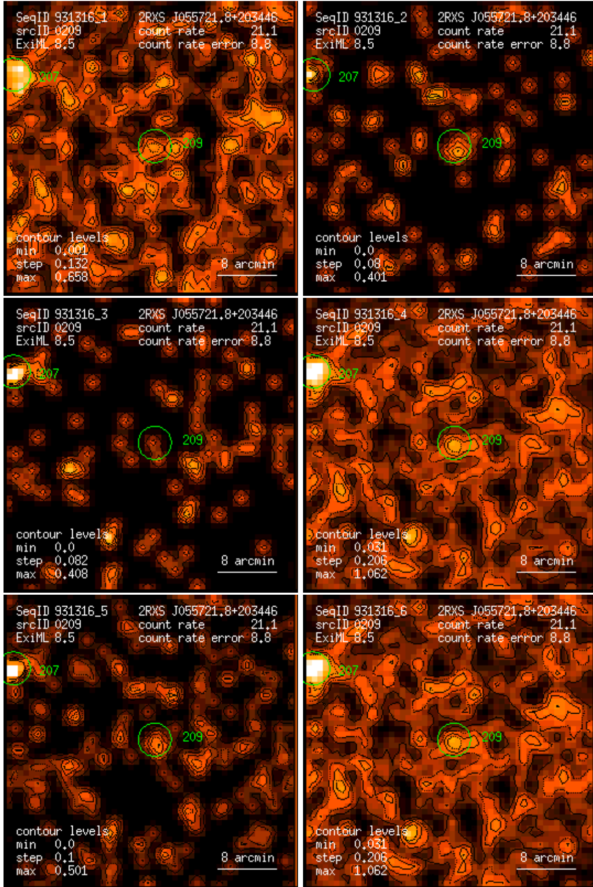
Figure 209: RASS 931316: detection 0209: band rate images, Gaussian filter: (1) PSPC channels 11 – 41, (2) 52 – 90, (3) 91 – 201, (4) 11 – 235, (5) 52 – 201, (6) 11 – 201. Broad band rates in counts/ks. Band rate contour levels in counts/ks/arcmin 2 .
