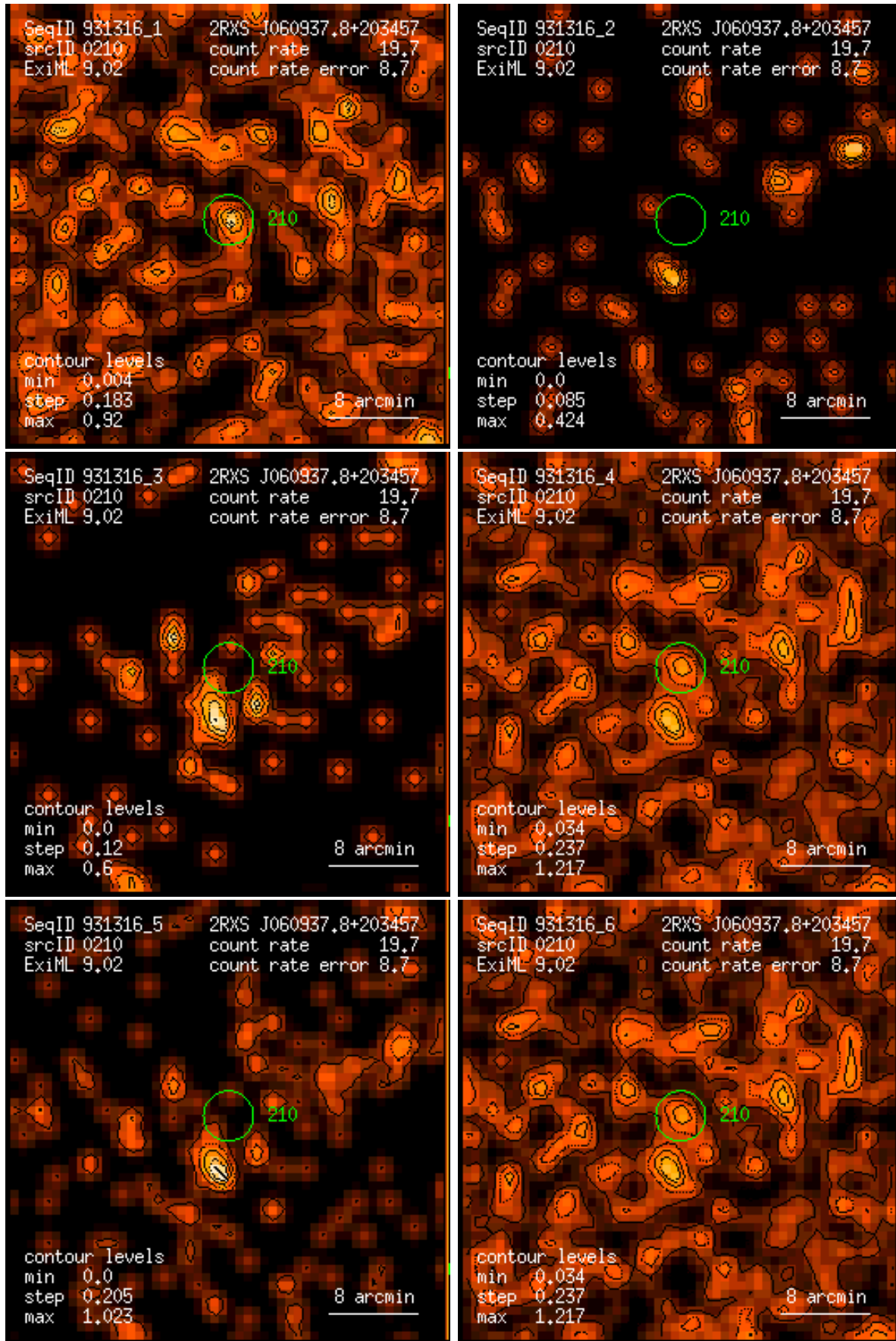
Figure 210: RASS 931316: detection 0210: band rate images, Gaussian filter: (1) PSPC channels 11 – 41, (2) 52 – 90, (3) 91 – 201, (4) 11 – 235, (5) 52 – 201, (6) 11 – 201. Broad band rates in counts/ks. Band rate contour levels in counts/ks/arcmin 2 .
