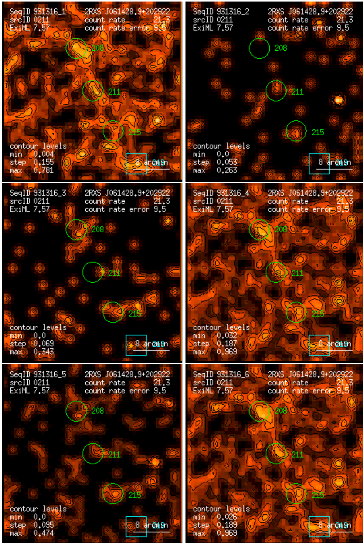
Figure 211: RASS 931316: detection 0211: band rate images, Gaussian filter: (1) PSPC channels 11 – 41, (2) 52 – 90, (3) 91 – 201, (4) 11 – 235, (5) 52 – 201, (6) 11 – 201. Broad band rates in counts/ks. Band rate contour levels in counts/ks/arcmin 2 .
