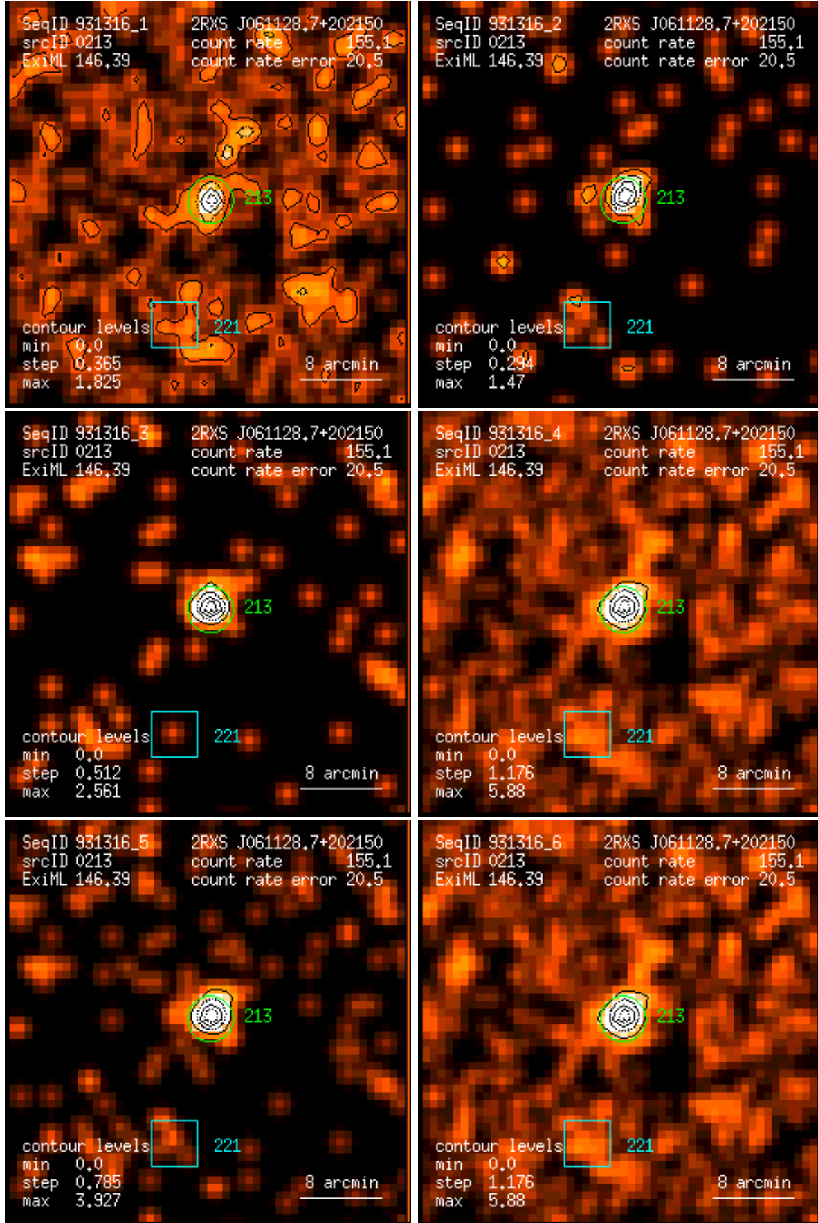
Figure 213: RASS 931316: detection 0213: band rate images, Gaussian filter: (1) PSPC channels 11 – 41, (2) 52 – 90, (3) 91 – 201, (4) 11 – 235, (5) 52 – 201, (6) 11 – 201. Broad band rates in counts/ks. Band rate contour levels in counts/ks/arcmin 2 .
