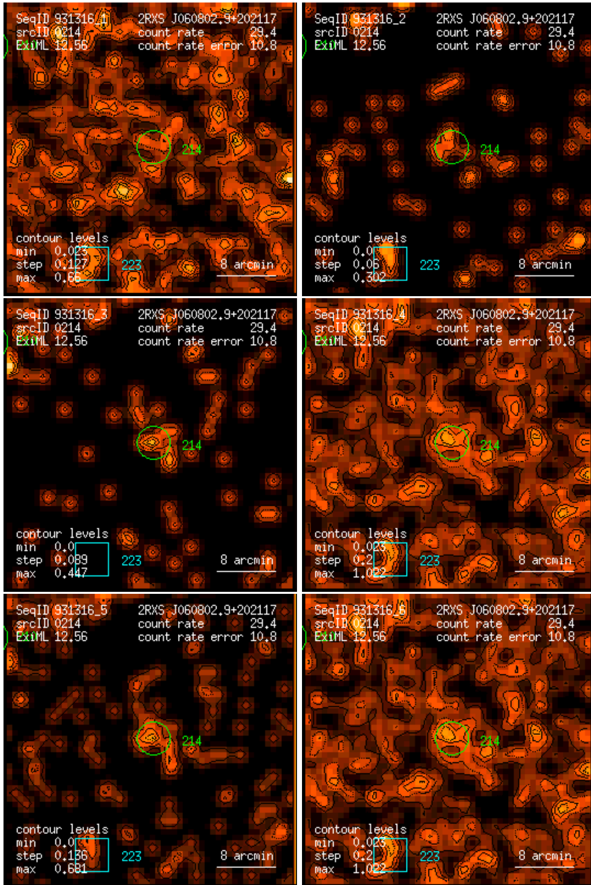
Figure 214: RASS 931316: detection 0214: band rate images, Gaussian filter: (1) PSPC channels 11 – 41, (2) 52 – 90, (3) 91 – 201, (4) 11 – 235, (5) 52 – 201, (6) 11 – 201. Broad band rates in counts/ks. Band rate contour levels in counts/ks/arcmin 2 .
