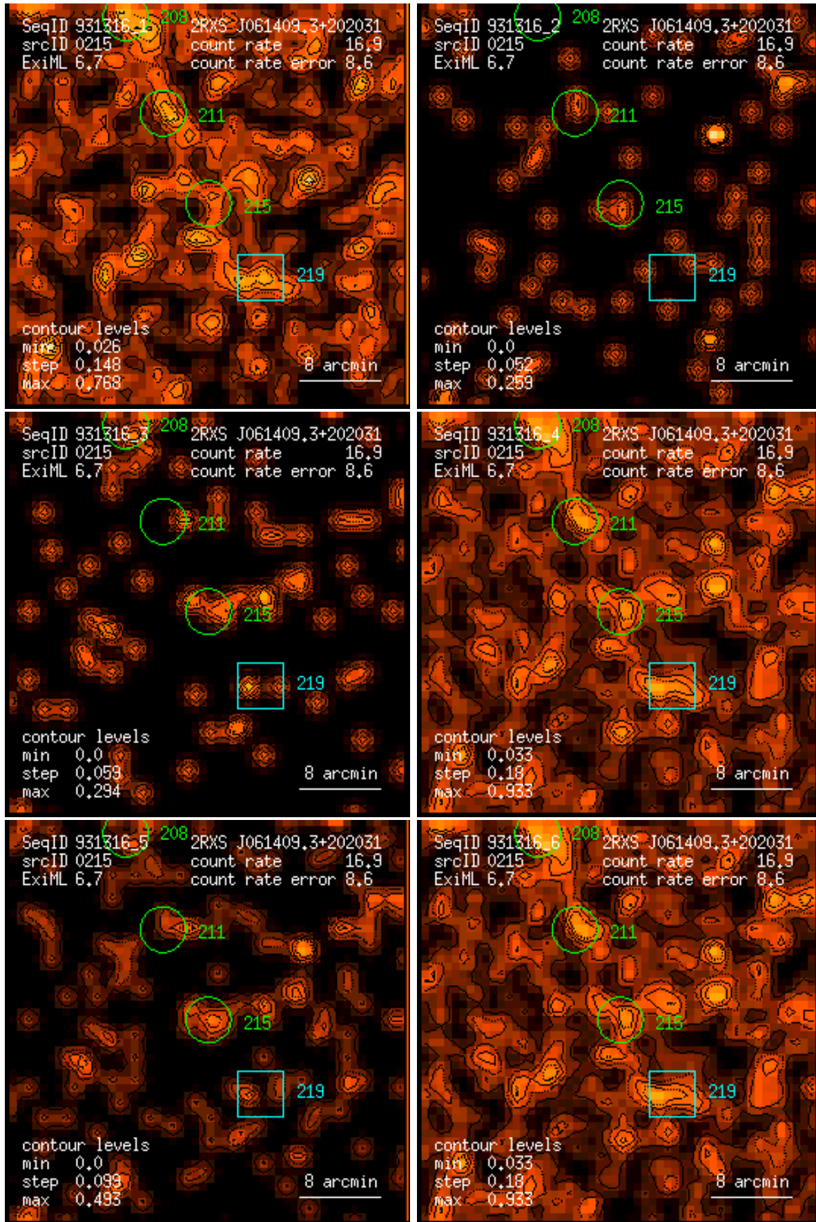
Figure 215: RASS 931316: detection 0215: band rate images, Gaussian filter: (1) PSPC channels 11 – 41, (2) 52 – 90, (3) 91 – 201, (4) 11 – 235, (5) 52 – 201, (6) 11 – 201. Broad band rates in counts/ks. Band rate contour levels in counts/ks/arcmin 2 .
