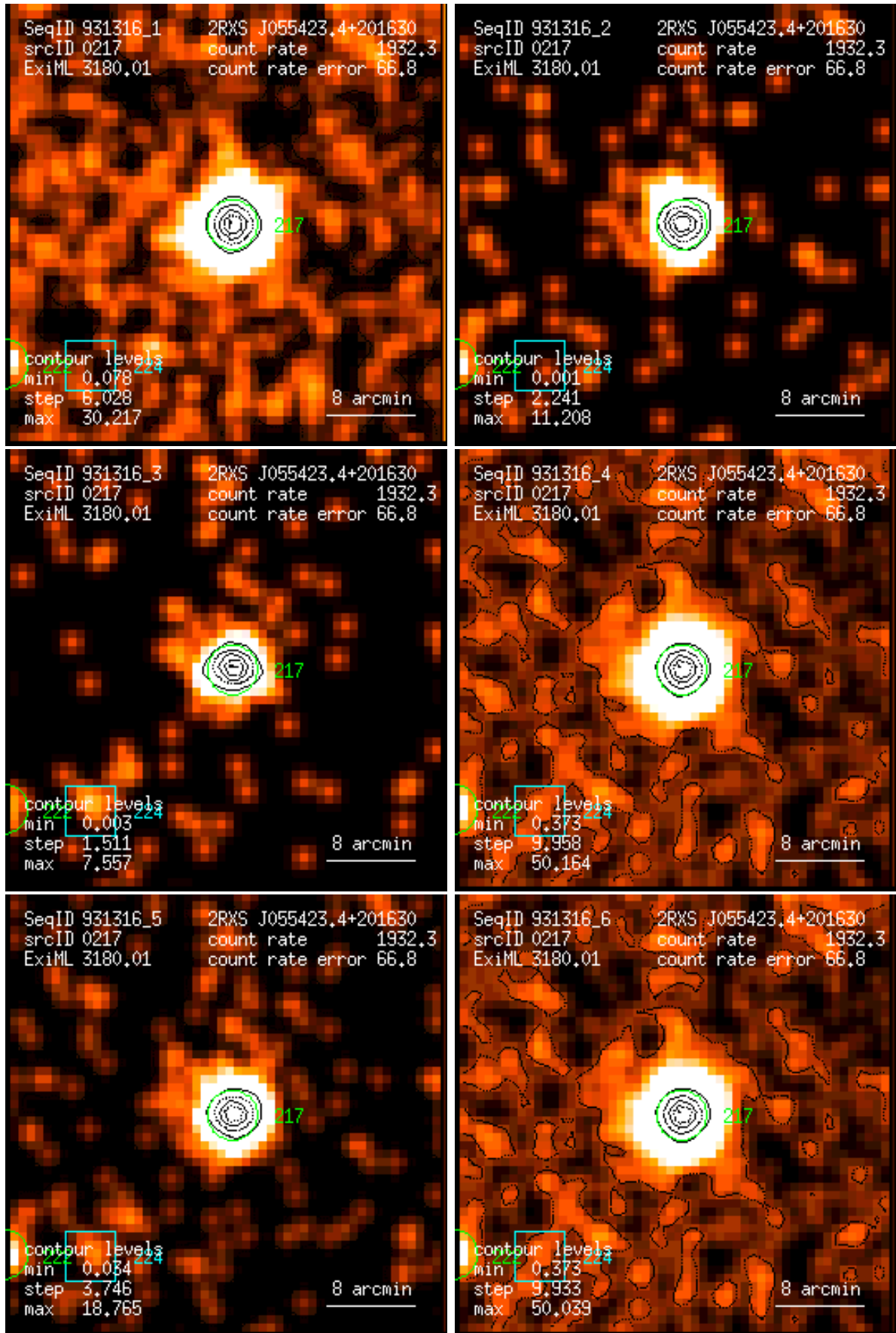
Figure 217: RASS 931316: detection 0217: band rate images, Gaussian filter: (1) PSPC channels 11 – 41, (2) 52 – 90, (3) 91 – 201, (4) 11 – 235, (5) 52 – 201, (6) 11 – 201. Broad band rates in counts/ks. Band rate contour levels in counts/ks/arcmin 2 .
