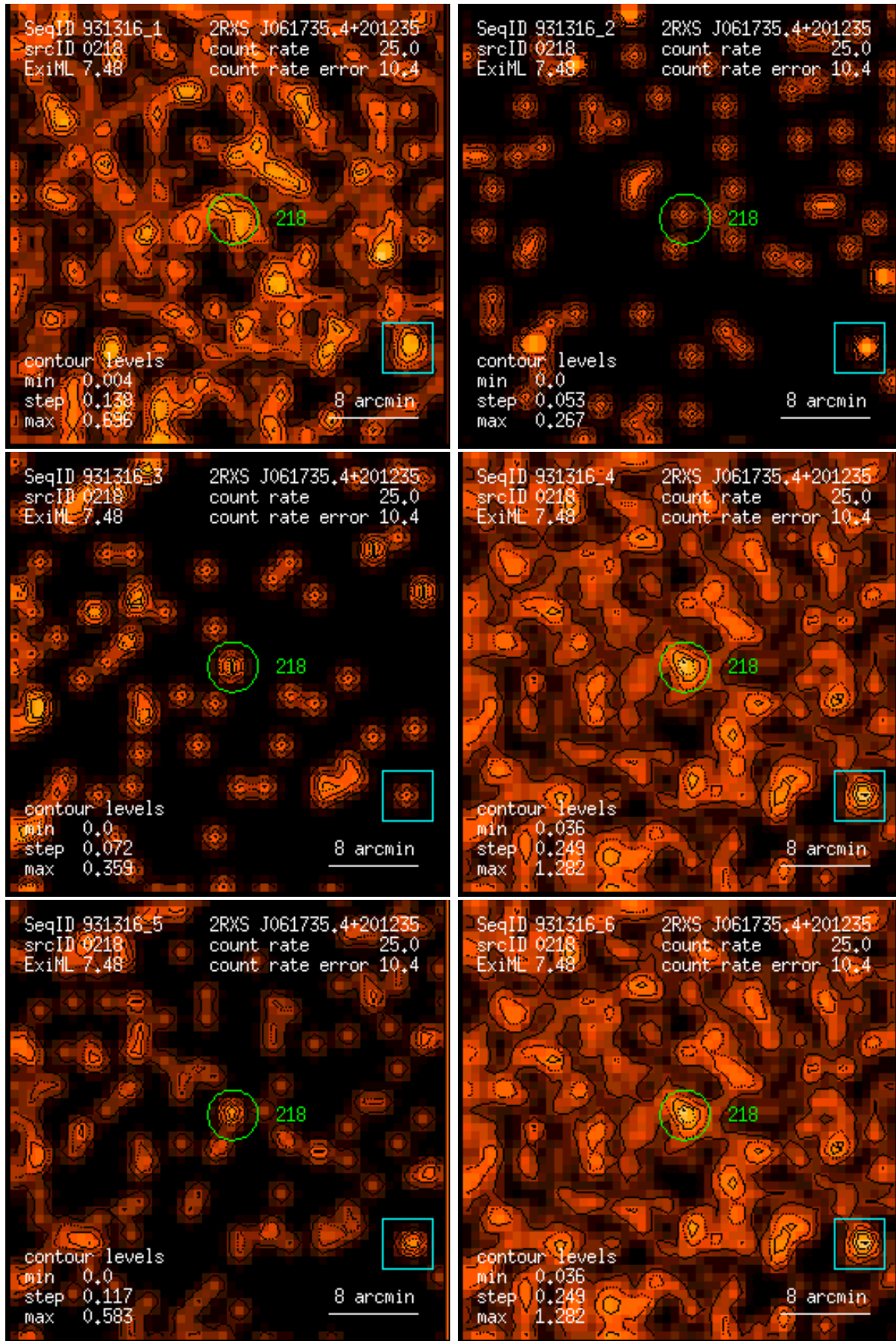
Figure 218: RASS 931316: detection 0218: band rate images, Gaussian filter: (1) PSPC channels 11 – 41, (2) 52 – 90, (3) 91 – 201, (4) 11 – 235, (5) 52 – 201, (6) 11 – 201. Broad band rates in counts/ks. Band rate contour levels in counts/ks/arcmin 2 .
