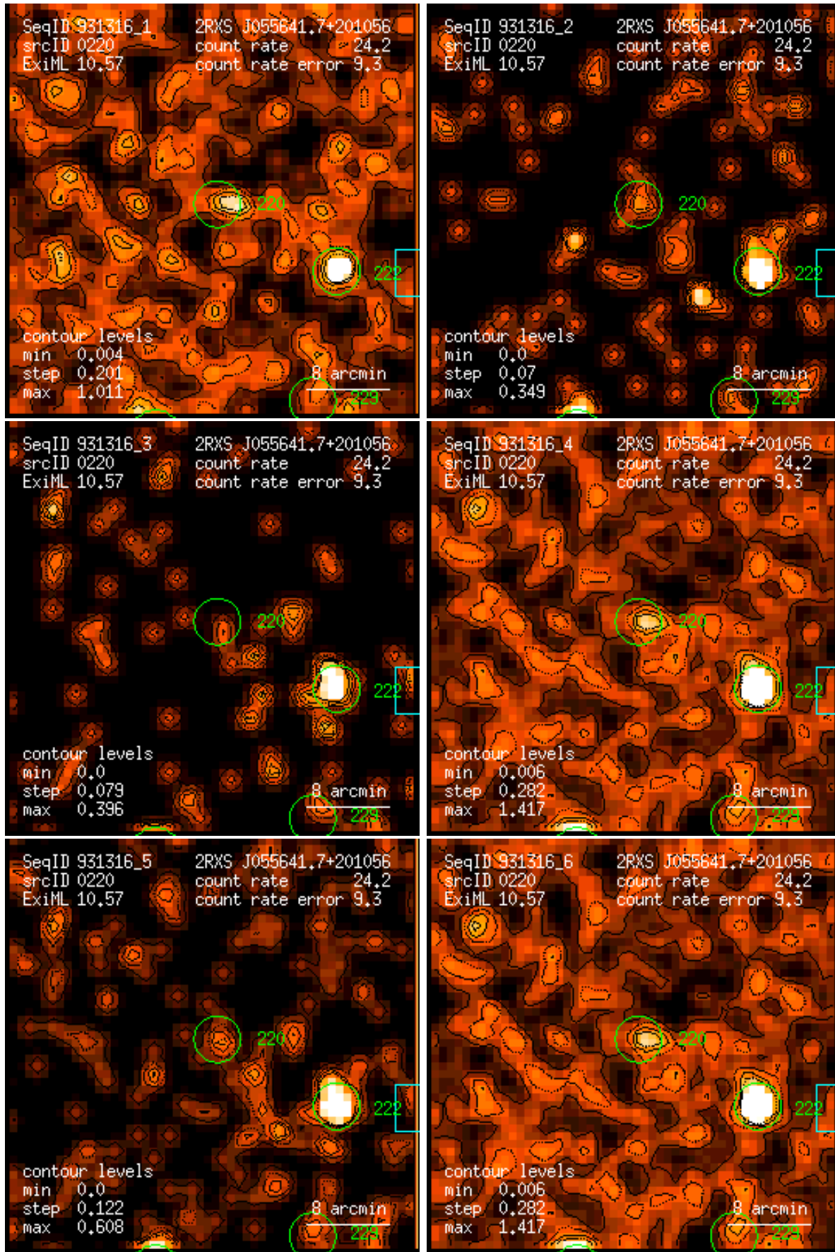
Figure 220: RASS 931316: detection 0220: band rate images, Gaussian filter: (1) PSPC channels 11 – 41, (2) 52 – 90, (3) 91 – 201, (4) 11 – 235, (5) 52 – 201, (6) 11 – 201. Broad band rates in counts/ks. Band rate contour levels in counts/ks/arcmin 2 .
