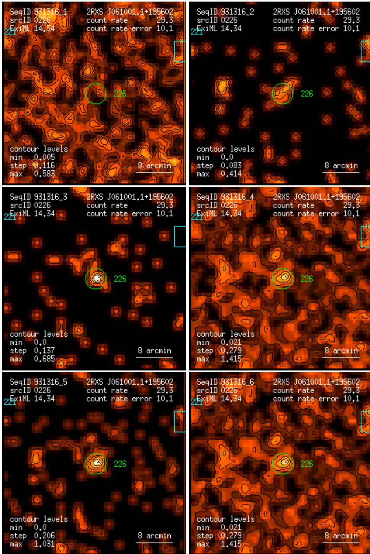
Figure 226: RASS 931316: detection 0226: band rate images, Gaussian filter: (1) PSPC channels 11 – 41, (2) 52 – 90, (3) 91 – 201, (4) 11 – 235, (5) 52 – 201, (6) 11 – 201. Broad band rates in counts/ks. Band rate contour levels in counts/ks/arcmin 2 .
