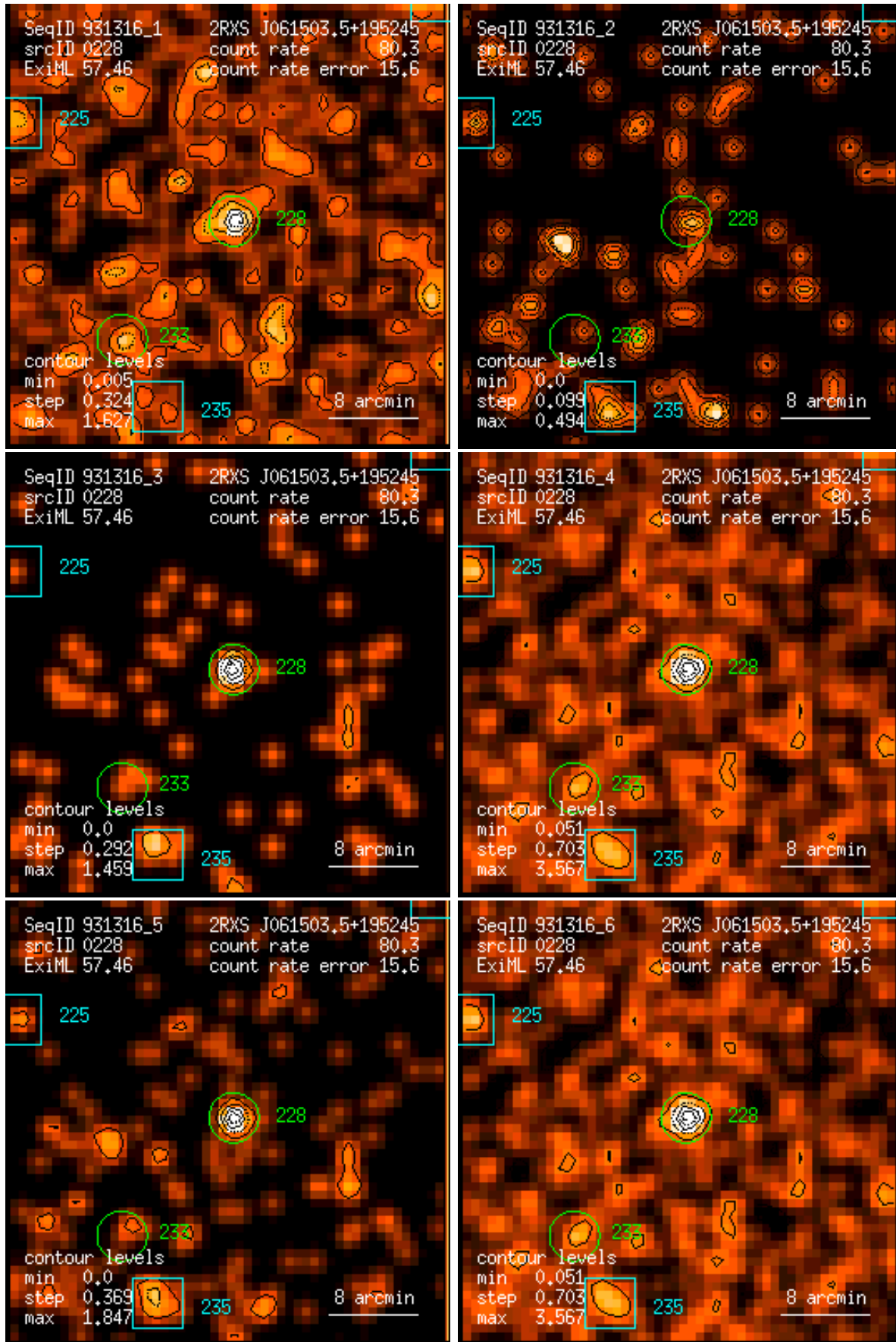
Figure 228: RASS 931316: detection 0228: band rate images, Gaussian filter: (1) PSPC channels 11 – 41, (2) 52 – 90, (3) 91 – 201, (4) 11 – 235, (5) 52 – 201, (6) 11 – 201. Broad band rates in counts/ks. Band rate contour levels in counts/ks/arcmin 2 .
