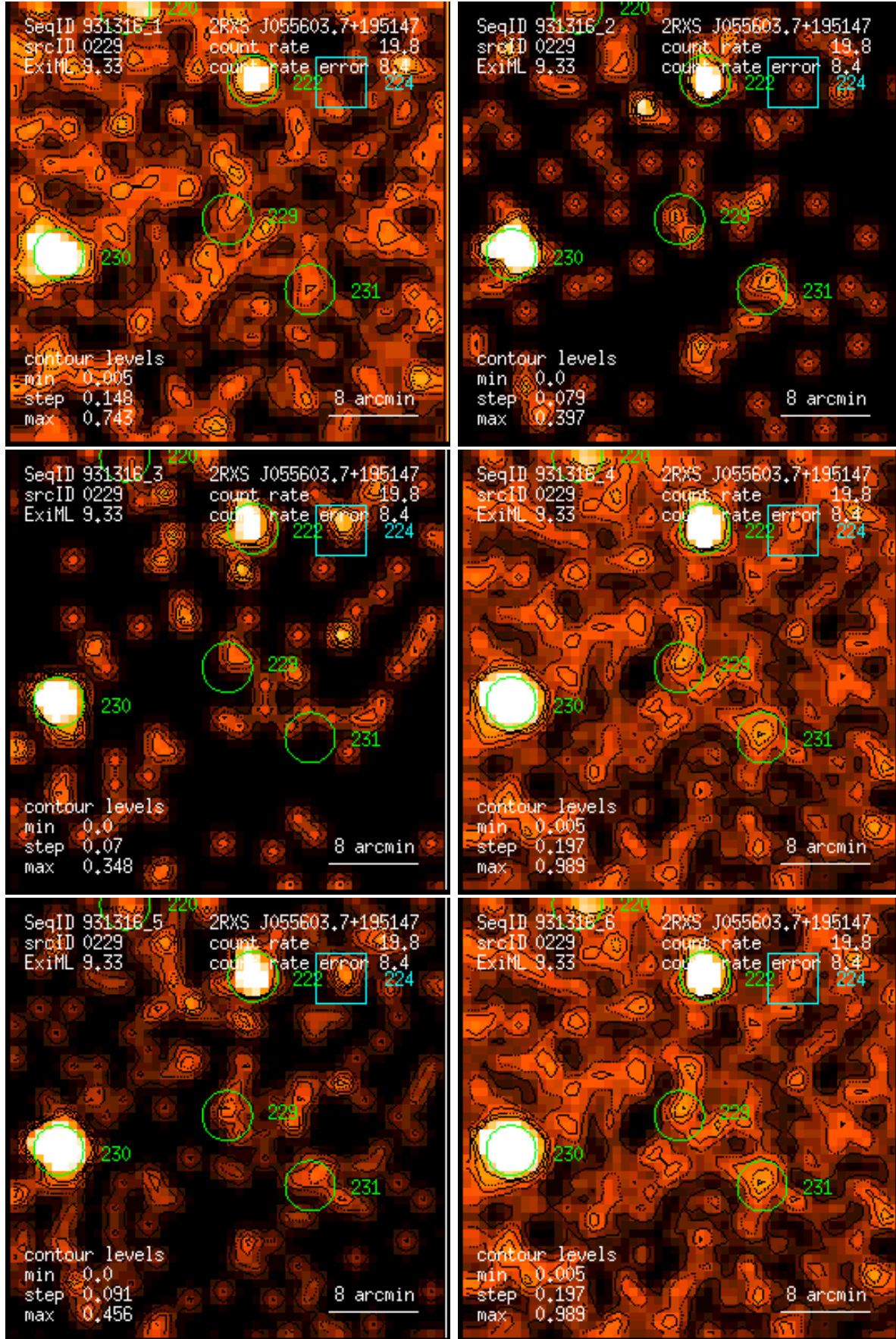
Figure 229: RASS 931316: detection 0229: band rate images, Gaussian filter: (1) PSPC channels 11 – 41, (2) 52 – 90, (3) 91 – 201, (4) 11 – 235, (5) 52 – 201, (6) 11 – 201. Broad band rates in counts/ks. Band rate contour levels in counts/ks/arcmin 2 .
