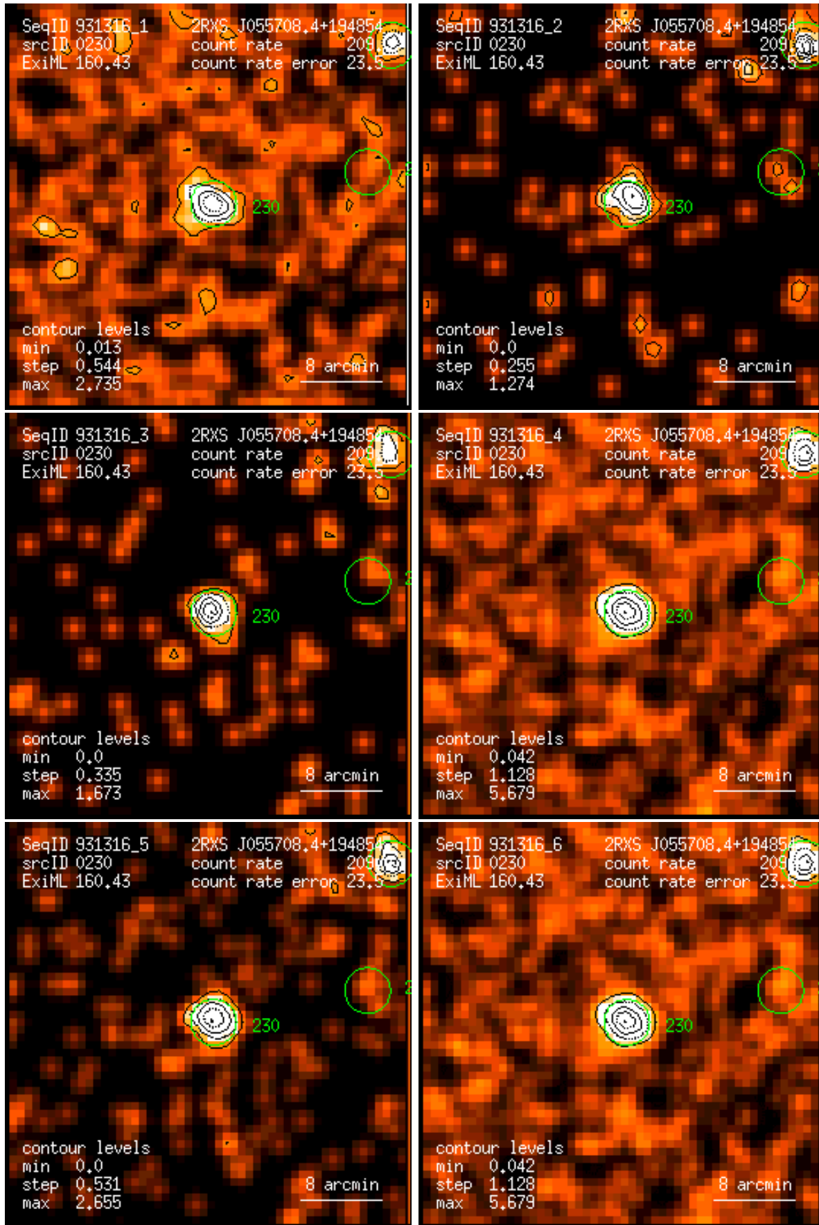
Figure 230: RASS 931316: detection 0230: band rate images, Gaussian filter: (1) PSPC channels 11 – 41, (2) 52 – 90, (3) 91 – 201, (4) 11 – 235, (5) 52 – 201, (6) 11 – 201. Broad band rates in counts/ks. Band rate contour levels in counts/ks/arcmin 2 .
