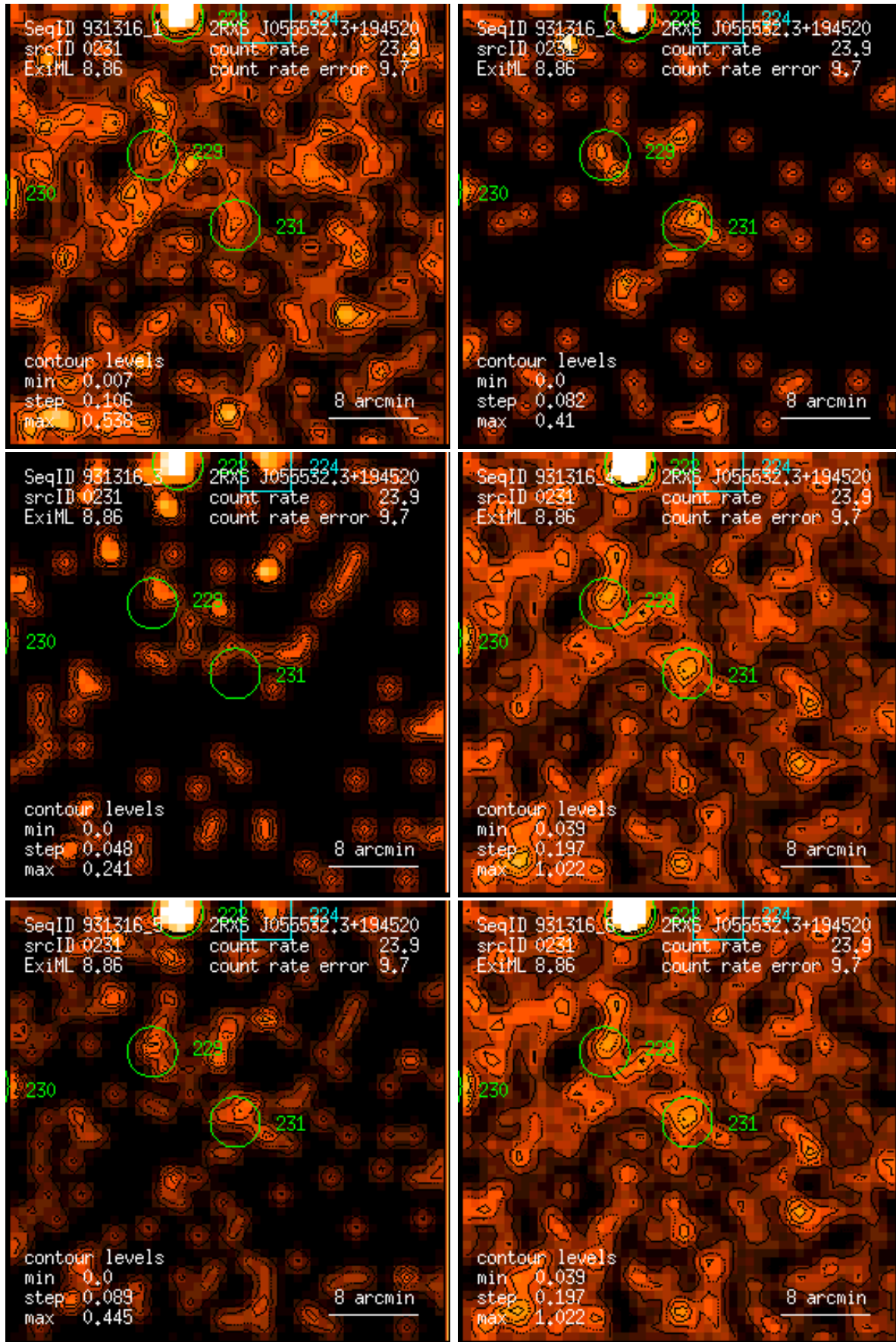
Figure 231: RASS 931316: detection 0231: band rate images, Gaussian filter: (1) PSPC channels 11 – 41, (2) 52 – 90, (3) 91 – 201, (4) 11 – 235, (5) 52 – 201, (6) 11 – 201. Broad band rates in counts/ks. Band rate contour levels in counts/ks/arcmin 2 .
