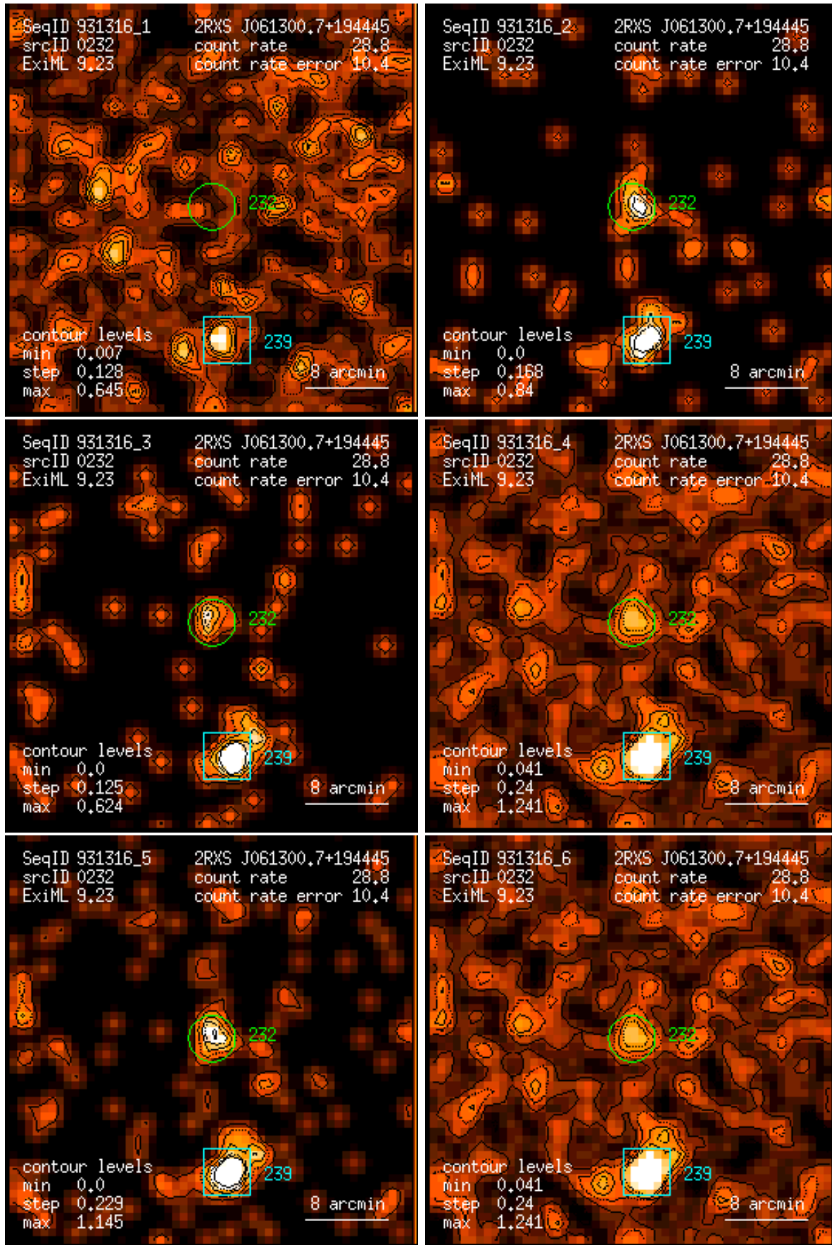
Figure 232: RASS 931316: detection 0232: band rate images, Gaussian filter: (1) PSPC channels 11 – 41, (2) 52 – 90, (3) 91 – 201, (4) 11 – 235, (5) 52 – 201, (6) 11 – 201. Broad band rates in counts/ks. Band rate contour levels in counts/ks/arcmin 2 .
