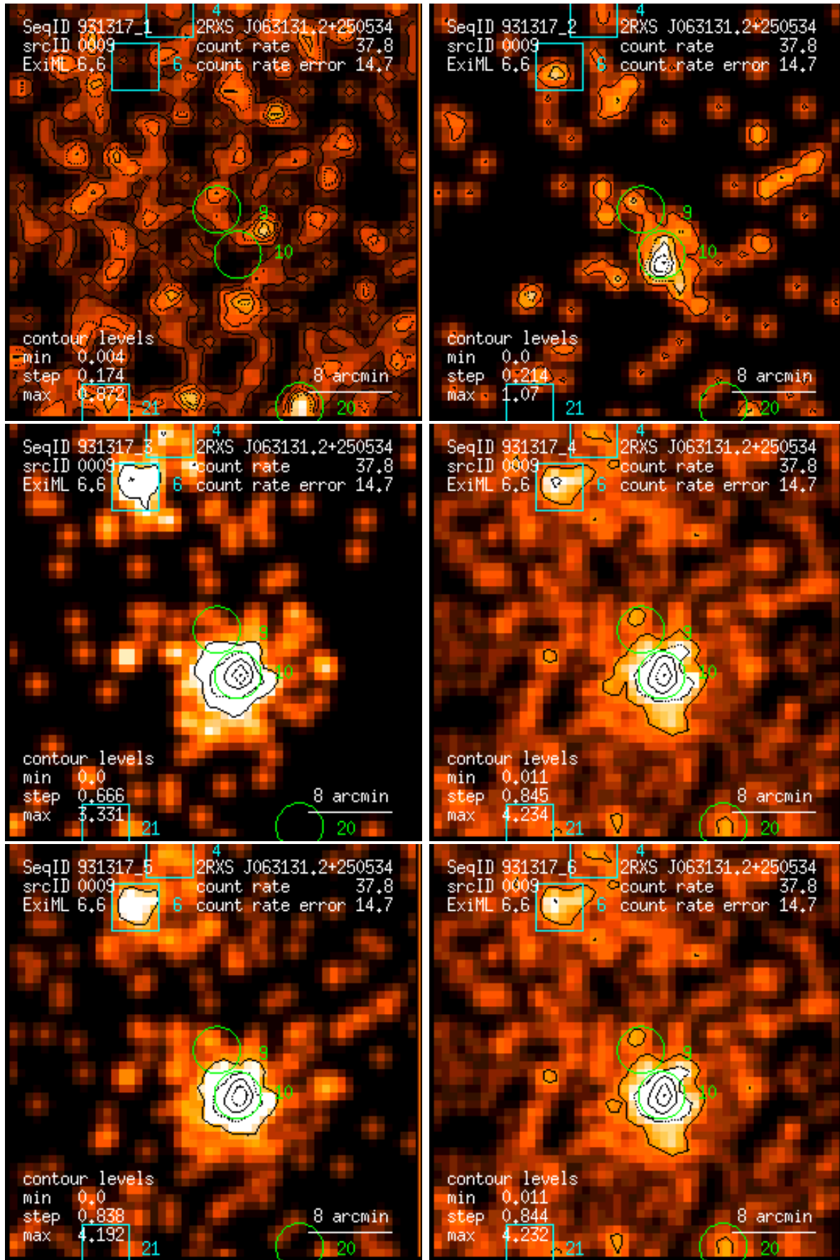
Figure 9: RASS 931317: detection 0009: band rate images, Gaussian filter: (1) PSPC channels 11 – 41, (2) 52 – 90, (3) 91 – 201, (4) 11 – 235, (5) 52 – 201, (6) 11 – 201. Broad band rates in counts/ks. Band rate contour levels in counts/ks/arcmin 2 .
