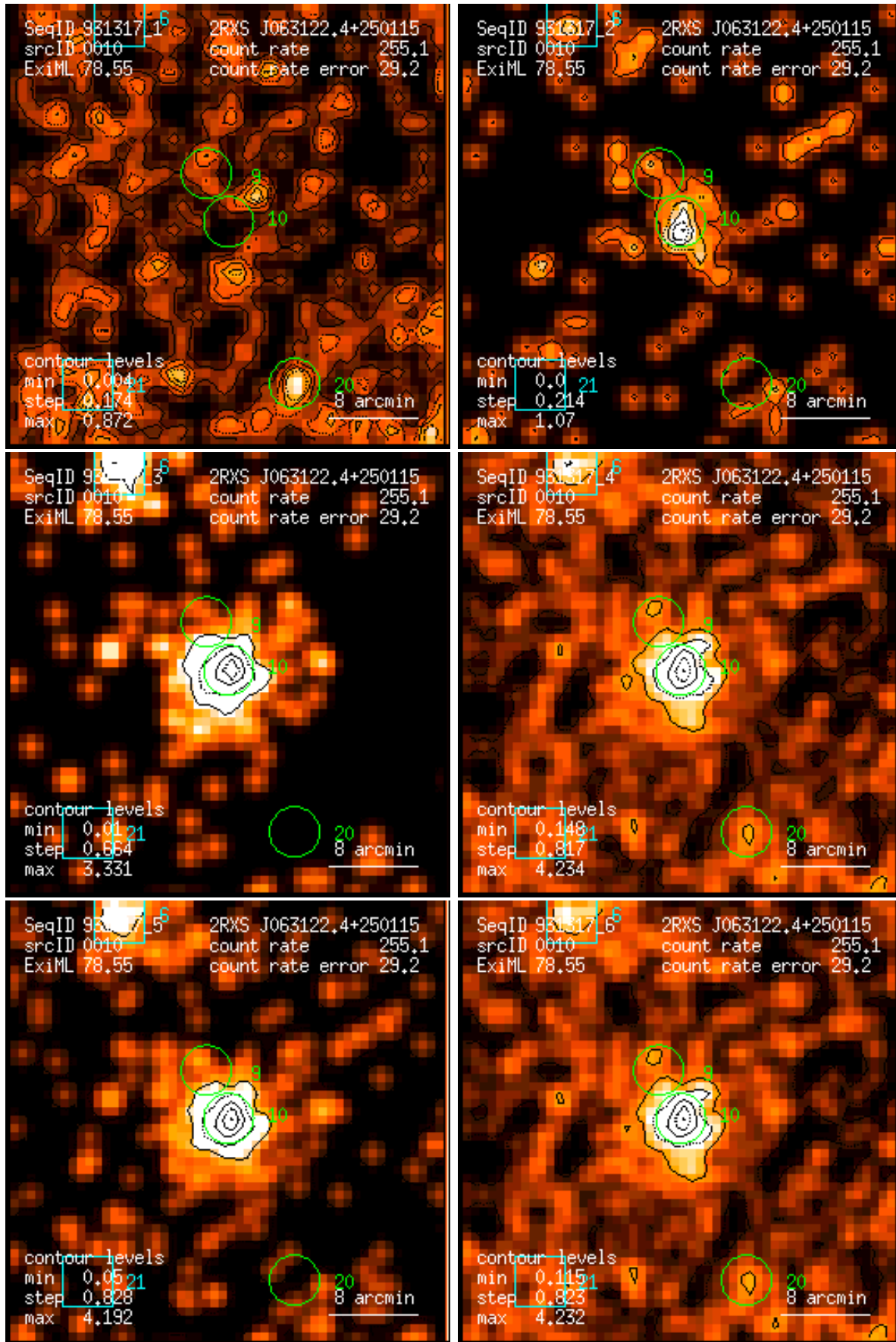
Figure 10: RASS 931317: detection 0010: band rate images, Gaussian filter: (1) PSPC channels 11 – 41, (2) 52 – 90, (3) 91 – 201, (4) 11 – 235, (5) 52 – 201, (6) 11 – 201. Broad band rates in counts/ks. Band rate contour levels in counts/ks/arcmin 2 .
