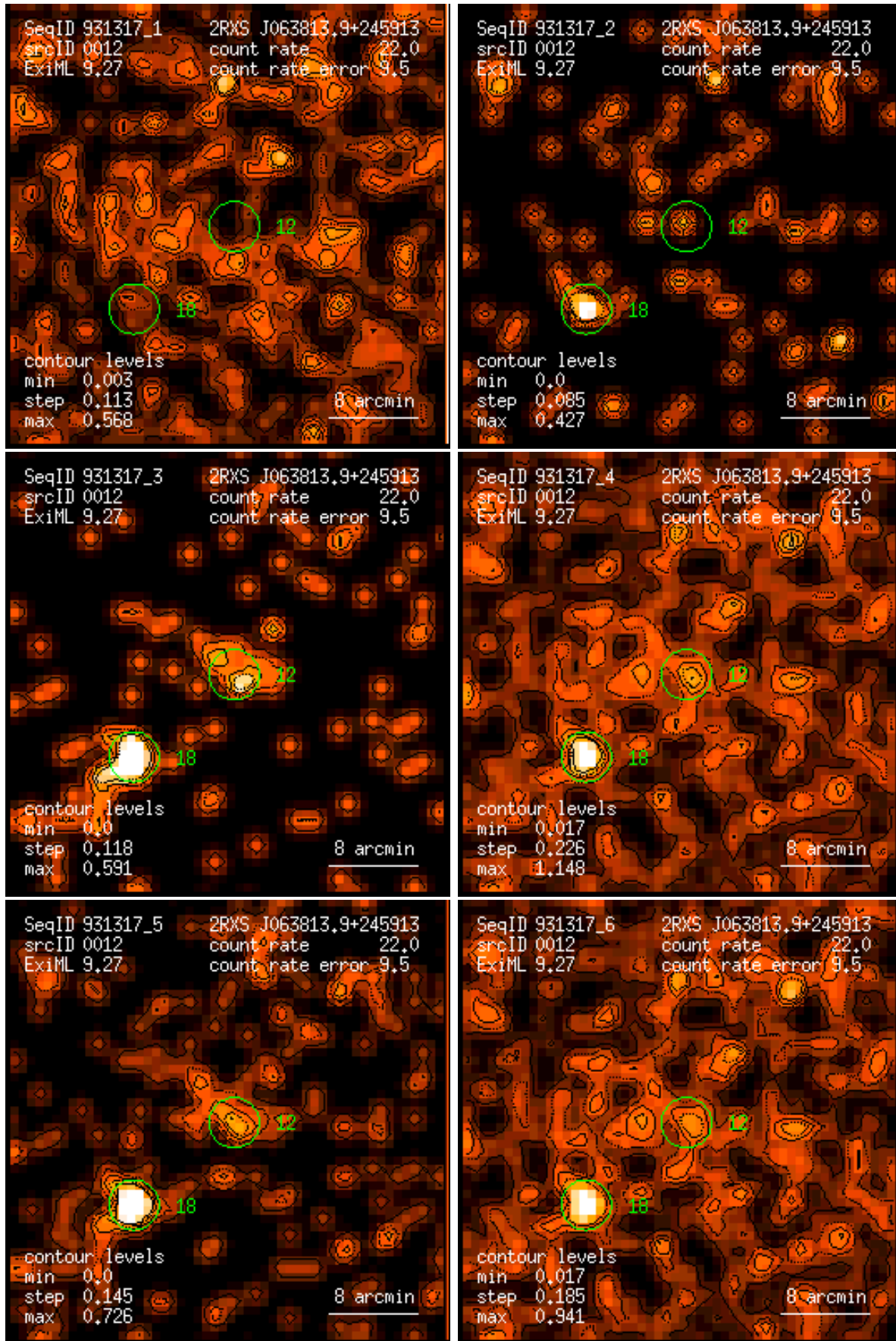
Figure 12: RASS 931317: detection 0012: band rate images, Gaussian filter: (1) PSPC channels 11 – 41, (2) 52 – 90, (3) 91 – 201, (4) 11 – 235, (5) 52 – 201, (6) 11 – 201. Broad band rates in counts/ks. Band rate contour levels in counts/ks/arcmin 2 .
