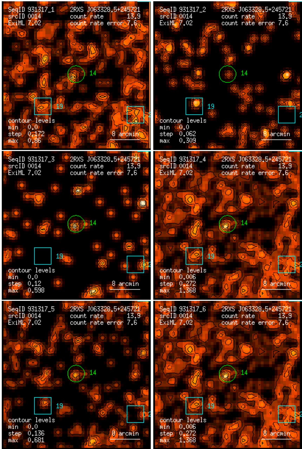
Figure 14: RASS 931317: detection 0014: band rate images, Gaussian filter: (1) PSPC channels 11 – 41, (2) 52 – 90, (3) 91 – 201, (4) 11 – 235, (5) 52 – 201, (6) 11 – 201. Broad band rates in counts/ks. Band rate contour levels in counts/ks/arcmin 2 .
