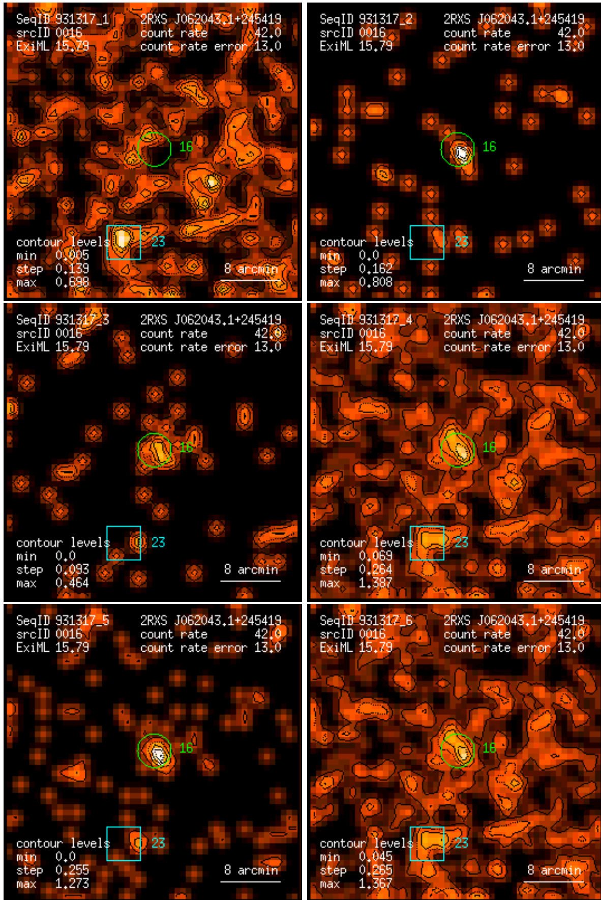
Figure 16: RASS 931317: detection 0016: band rate images, Gaussian filter: (1) PSPC channels 11 – 41, (2) 52 – 90, (3) 91 – 201, (4) 11 – 235, (5) 52 – 201, (6) 11 – 201. Broad band rates in counts/ks. Band rate contour levels in counts/ks/arcmin 2 .
